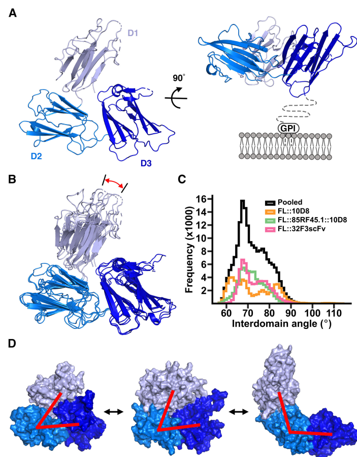
Figure 3: Structure and dynamics of Pfs48/45
