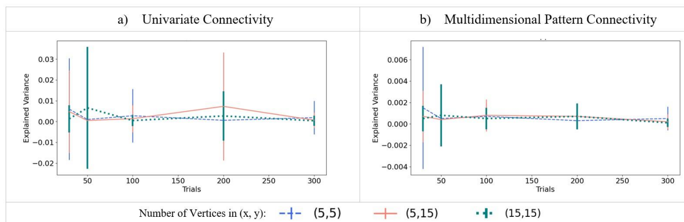
Figure 3- Estimating connectivity (explained variance) between two independent activity patterns, i.e., simulated regions without true connectivity, using MDPC and the UVC approach. a) Connectivity measured using the UVC method as a function of the different numbers of trials, for three different combinations of number of vertices in ROI X and ROI Y. b) Similar to a), but for the MDPC method. Both UVC and MDPC methods show connectivity scores close to zero, i.e., they do not produce false positives for independent patterns in the two regions. Error bars reflect standard deviations.
