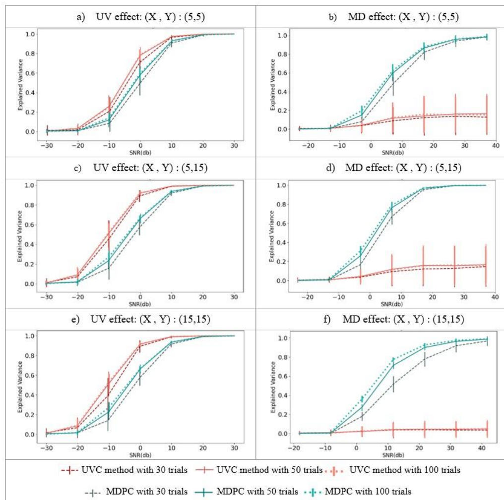
Figure 4- Comparing the MDPC and univariate connectivity (UVC) approaches on the detection of univariate (left panels) and multidimensional (right panels) relationships. All panels show explained variance (y-axis) across different SNRs (x-axis) for the MDPC (blue) and UVC (red) approaches with different numbers of trials (darker versus lighter shades of blue or red). a, c, e) show the connectivity scores for simulated activity patterns with a univariate dependency. In all cases, EV approaches 1 for SNRs greater than 10db, and is almost zero for SNRs below -25db. Both UVC and MDPC methods capture univariate relationships in medium-to-high SNRs, with greater EV for UVC. b, d, f) represent connectivity scores between patterns with a multidimensional dependency. For the MDPC method, EV approaches 1 for SNRs greater than 20db, and is almost zero for SNRs below -10db. For the UVC approach, the EV never exceeds a variance of 0.2, and is almost zero below -10db. Error bars reflect standard deviations.
