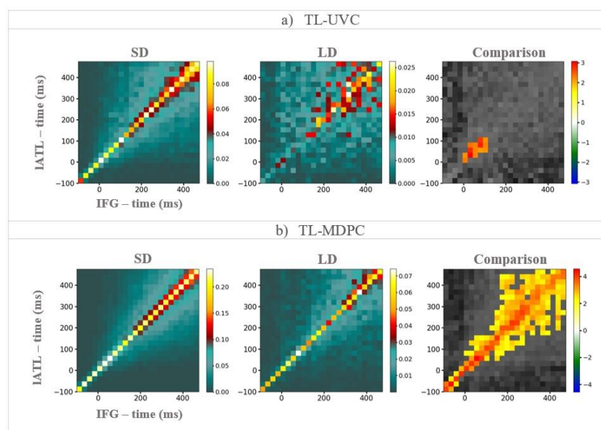
Figure 5- An example of TTMs showing the connectivity between the left ATL (y-axis) and IFG (x-axis), for the semantic decision (SD) task (the left column), the lexical decision (LD) task (the middle column), and their comparison (the right column) for which cluster size was thresholded at 12 cells. a) TTMs obtained using the time-lagged univariate connectivity (TL-UVC) approach demonstrate some modulation between the two tasks at a limited number of time points early in processing. b) TTMs obtained using the TL-MDPC method. Here, there is a wider pattern of significant task differences across the trial with prediction possible across longer lags. The upper diagonal indicates statistical dependencies where the lATL is ahead in time, and the lower part shows dependencies where the IFG is ahead in time, capturing different information. Colorbars show connectivity scores for the first two columns and t-values for the third column. Note, the matrices have idiosyncratic scales for display purposes, and the connectivity values are greater for the TL-MDPC method than the TL-UVC approach.
