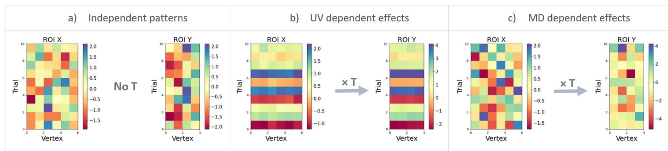
Figure 2- Illustration of different connectivity scenarios used in our simulations. The matrices illustrate activity patterns in regions X and Y , with rows representing different trials and columns representing vertices. a) X and Y contain random patterns. Thus, there is no reliable transformation between the patterns and consequently no connectivity. b) Patterns in X and Y have a univariate relationship. The amplitudes of patterns in the two regions covary linearly across trials (plus added noise). c) Patterns in X and Y have a multidimensional relationship. The patterns in Y were obtained by applying a linear transformation matrix to the patterns in X (plus noise).
