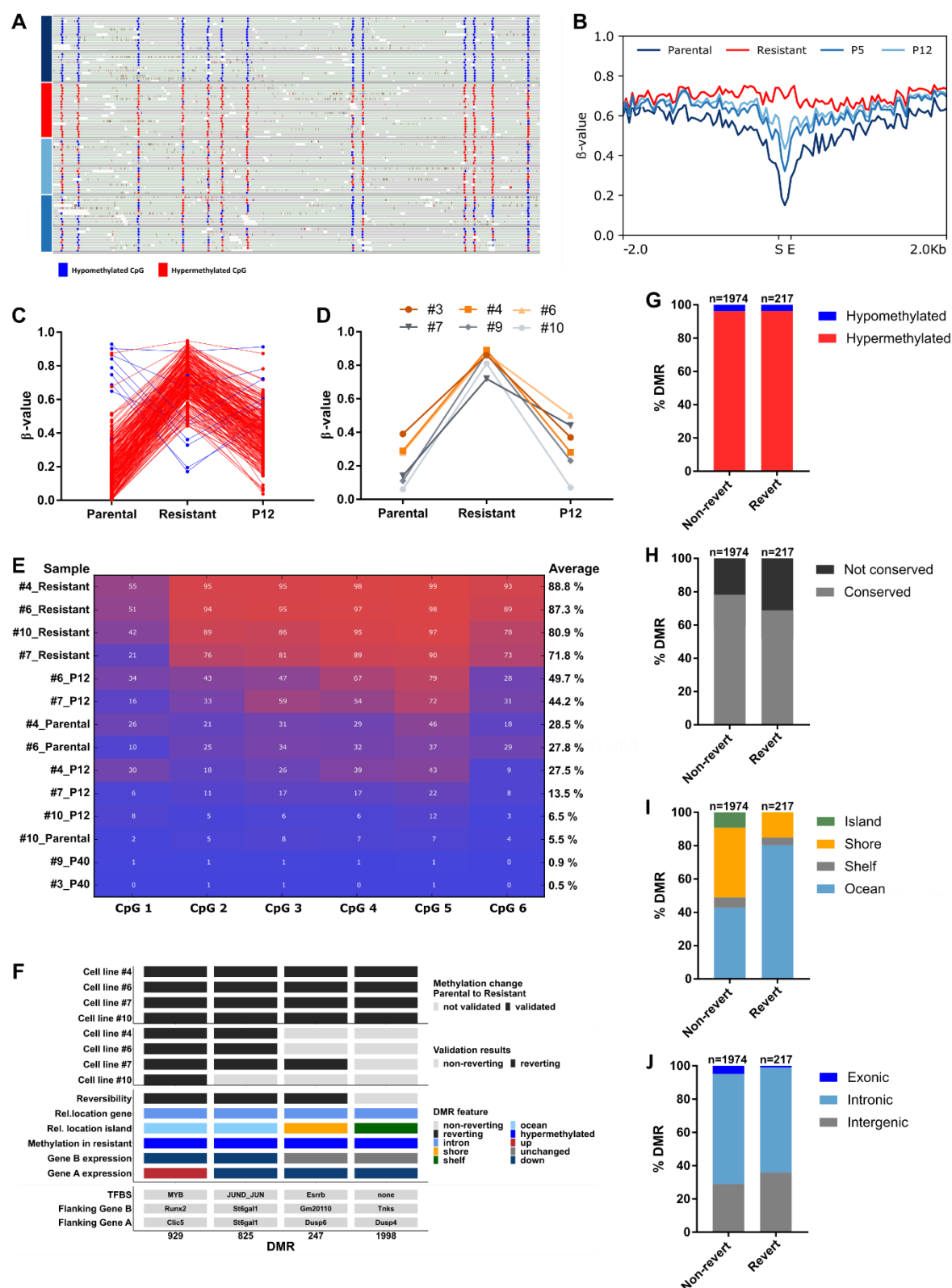
Fig. 4. Distinct DMRs revert after MEK i withdrawal
