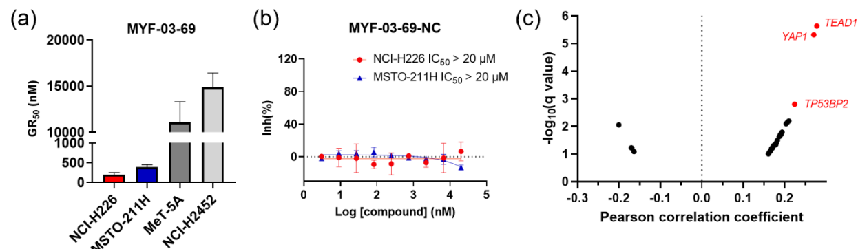
Figure S9 | (a) The calculated GR 50 values of MYF-03-69 in 5-day proliferation assay on mesothelioma cells. NCI-H226 and MSTO-211H are Hippo signaling defective mesothelioma cells. NCI-H2452 is Hippo signaling intact mesothelioma cell. MeT-5A is non-cancerous mesothelium cell. This figure is related to Figure 5a . (b) MYF-03-69-NC did not inhibit cell proliferation of NCI-H226 and MSTO-211H cells in 5-day treatment. This figure is related to Figure 5a . (c) Correlation analysis between compound PRISM sensitivity (log 2 .AUC of each cell line) and dependency of certain gene (CRISPR knockout score for each cell line, from DepMap Public 20Q4 Achilles_gene_effect.csv dataset) across the PRISM cell line panel. The Pearson correlation coefficients (X axis) and associated p-values were computed. Positive correlations correspond to dependency correlating with increased sensitivity. The q-values (a corrected significance value accounting for false discovery rate) are computed from p-values using the Benjamini Hochberg algorithm. Associations with q-values above 0.1 are filtered out. Top 3 correlated genes are in red. Details are in Supplementary Dataset 4 .
