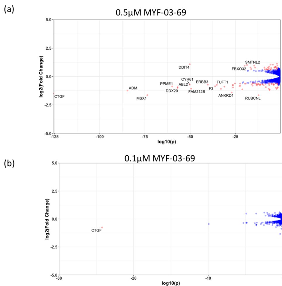
Figure S8 | The number of genes with significantly altered expression level decreased with lower concentration treatment in NCI-H226 cells. (a) 0.5 μM MYF-
