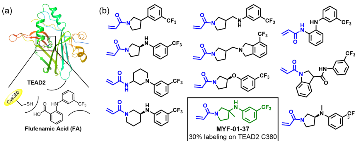
Figure S2 | Rationale of covalent fragments design. (a) Binding model of FA in TEAD2 palmitate pocket. (b) Chemical structures of representative covalent fragments. This figure is related to Figure 1a .
