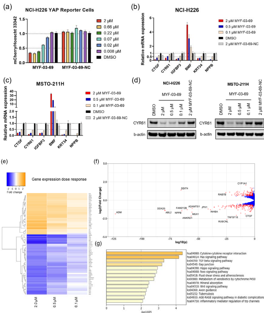
Figure 4 | MYF-03-69 inhibits YAP-TEAD transcription. (a) MYF-03-69, but not MYF-03-69-NC, inhibits YAP-TEAD transcriptional activity in NCI-H226 mCherry reporter cells. Cells were treated for 72 hours. (b-c) MYF-03-69, but not MYF-03-69-NC, downregulates YAP target genes and upregulates a pro-apoptotic gene BMF . Cells were treated for 24 hours. Data were presented as mean \pm SD of n = 3 biological independent samples. (d) MYF-03-69, but not MYF-03-69-NC, downregulates CYR61 protein level in NCI-H226 and MSTO-211H cells. (e) Heatmap for gene
