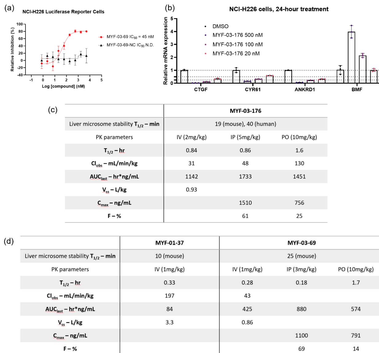
Figure S10 | (a) MYF-03-69, but not MYF-03-69-NC, inhibits YAP-TEAD transcriptional activity in NCI-H226 luciferase reporter cells. This figure is related to Figure 6b-c . (b) MYF-03-176 downregulates YAP target genes and upregulates a pro-apoptotic gene BMF . (c-d) Liver microsome stability and PK parameters comparison of MYF-03-176, MYF-03-69 and MYF-01-37.
