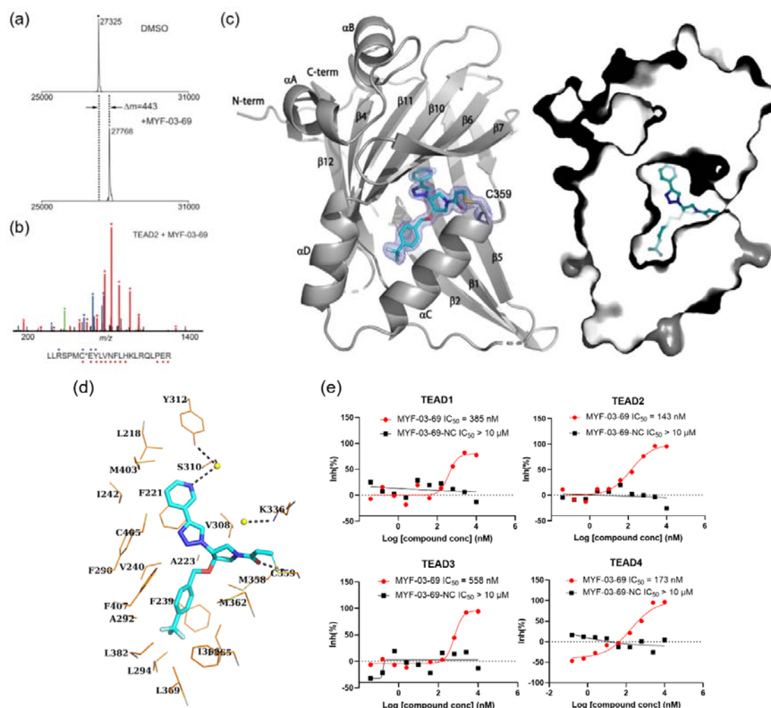
Figure 2 | MYF-03-69 binds in TEAD palmitate pocket covalently through the conserved cysteine. (a) The mass labeling of intact TEAD2 protein by MYF-03-69. (b) Trypsin digestion and tandem mass spectrum (MS/MS) localize labeling site of cysteine 380. (c) Co-crystal structure of MYF-03-69 with TEAD1 indicates covalent bond formation with Cys359. The compound adopts Y-shape and binds in both lipid tunnel and hydrophilic side pocket. (d) Interactions between MYF-03-69 and TEAD1 palmitate pocket. (e) A dose titration of MYF-03-69 and MYF-03-69-NC in anti-palmitoylation assay on TEAD1-4. Recombinant YBD protein of TEADs were preincubated with compounds at 37°C for 2 hours. Data are representative of n = 3 independent experiments.
