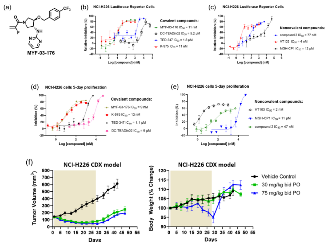
Figure 6 | MYF-03-176 is a potent and orally bioavailable YAP-TEAD transcription inhibitor and suppresses tumor growth in mesothelioma xenograft mouse model. (a) Chemical structure of MYF-03-176. (b-c) Inhibitory effect of MYF-03-176 and other TEAD PBP binders on YAP-TEAD transcription in NCI-H226 luciferase reporter cells. Cells were treated for 72 hours. Data were presented as mean \pm SD of n = 3 biological independent samples. (d-e) Antiproliferation effect of MYF-03-176 and other TEAD PBP binders in NCI-H226 cells. Cells were treated for 5 days. Data were presented as mean \pm SD of n = 3 biological independent samples. (f) In vivo efficacy of MYF-03-176 in NCI-H226 CDX mouse model (n = 8~9 per group).
