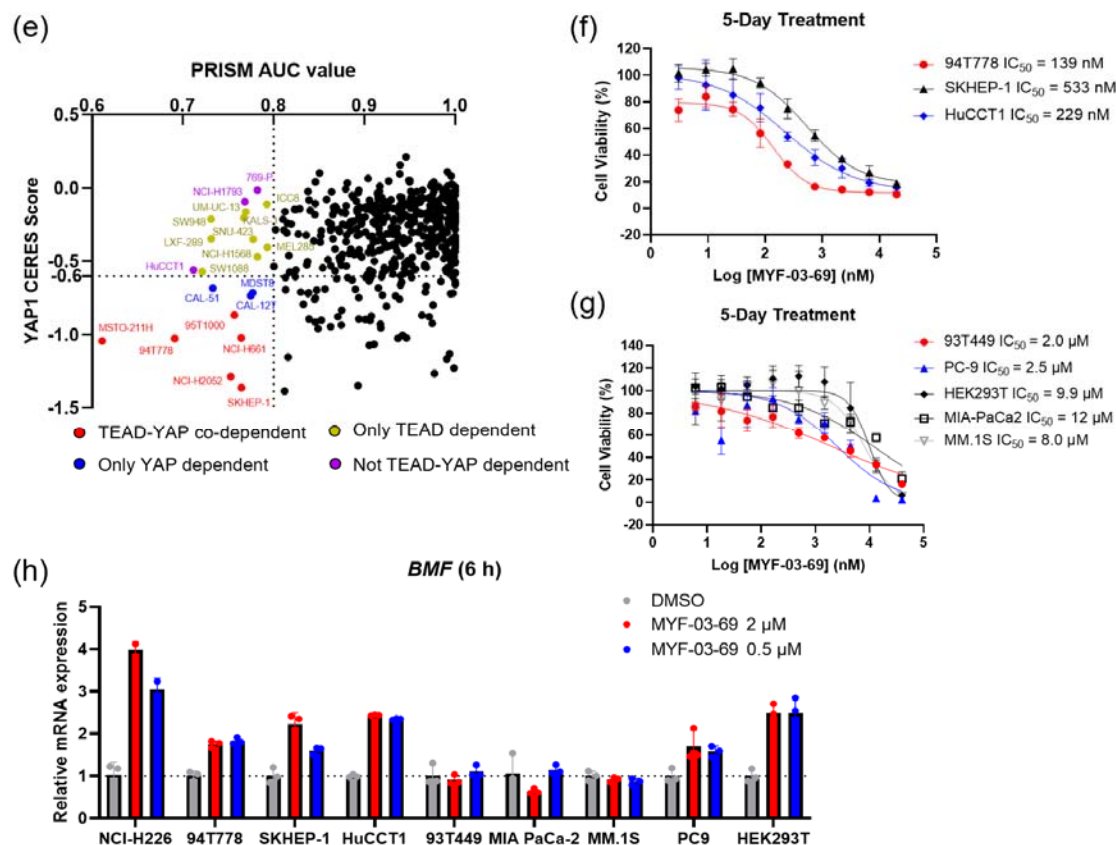
Figure 5 | MYF-03-69 selectively inhibits proliferation of cancer cells with YAP or TEAD dependency regardless of lineage. (a) Antiproliferation IC_{50} curve of MYF-03-69 on three mesothelioma cell lines (NCI-H226, MSTO-211H and NCI-H2452) and a normal noncancerous mesothelium cell line (Met-5A). (b) Antiproliferation IC_{50} curve of MYF-03-69 and MYF-03-69-NC in 3D cell culture. (c-d) Cell cycle arrest induced by MYF-03-69, but not MYF-03-69-NC. Cells were treated for 48 hours at indicated doses. (e) PRISM profiling across a broad panel of cell lineages. 903 cancer cells were treated with MYF-03-69 for 5 days. The viability values were measured at 8-point dose manner (3-fold dilution from 10 \mu M) and fitted a dose-response curve for each cell line. Area under the curve (AUC) was calculated as a measurement of compound effect on cell viability. CERES score of YAP1 or TEADs from CRISPR (Avana) Public 21Q1 dataset (DepMap) were used to estimate gene-dependency. Cell lines without CERES Score of YAP1 were excluded from the figure. The CERES Score of most dependent TEAD isoform was used to represent TEAD dependency. Cell lines with a dependency score less than -0.6 were defined as the dependent cell lines. (f) Antiproliferation curves of cell lines that are sensitive to MYF-03-69 treatment besides mesothelioma.
