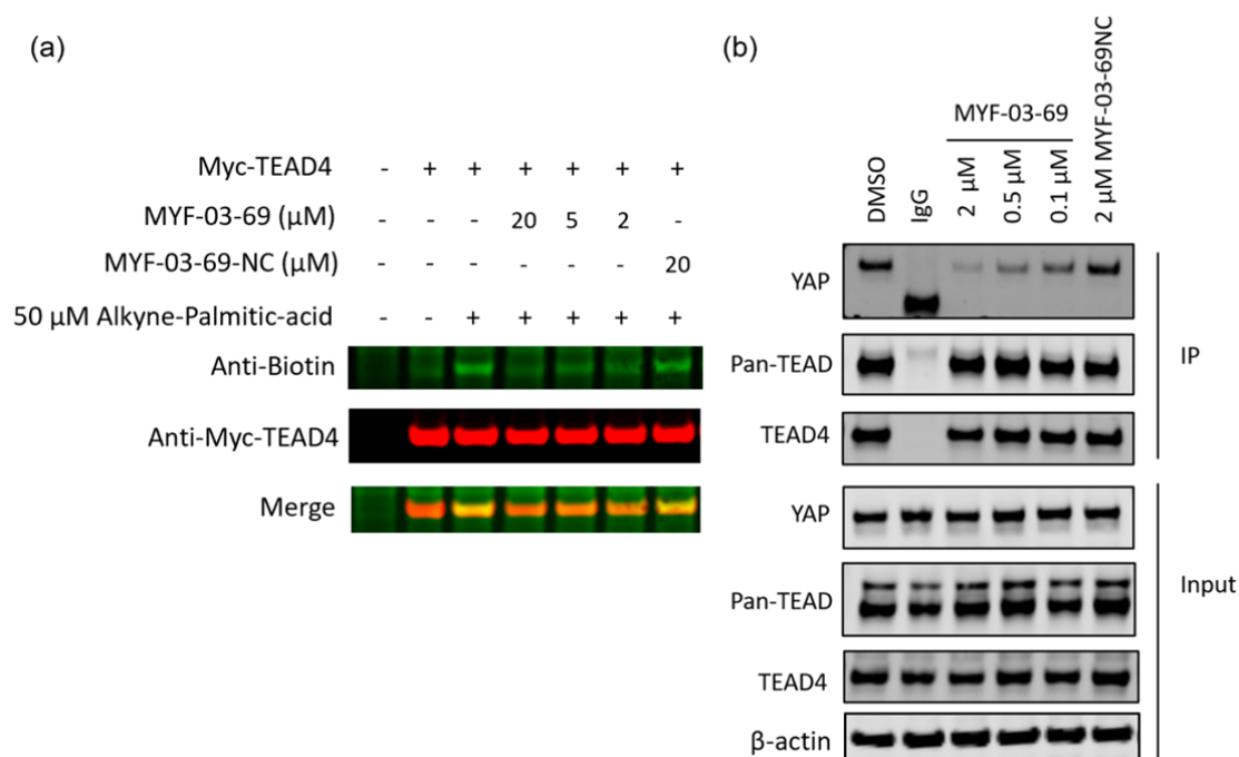
Figure 3 | MYF-03-69 inhibits palmitoylation of TEAD protein and disrupts its association with YAP in cells. (a) Palmitoylation of Myc-TEAD4 in HEK293T cells after treatment with MYF-03-69 and MYF-03-69-NC indicated by an alkyne-palmitic-acid probe and click chemistry. Cells were treated for 24 hours. (b) Co-immunoprecipitation (Co-IP) of endogenous YAP and TEAD in NCI-H226 cells after treatment with MYF-03-69 and MYF-03-69-NC at indicated doses. Cells were treated for 24 hours.
