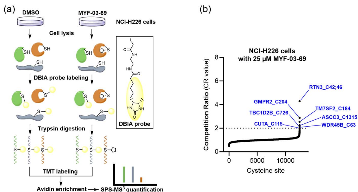
Figure S5 | MYF-03-69 exhibited low reactivity towards the cysteine proteome. (a) Overview of the SLC-ABPP proteome-wide selectivity approach for profiling of MYF-03-69. NCI-H226 cells were treated with 0.5, 2, 10 or 25 \mu M MYF-03-69 and DMSO over 3 hours in triplicates before cell lysis followed by labeling with DBIA probe. The SLC-ABPP approach was used to profile competition of MYF-03-69 in proteome cysteine labeling. Competition ratio (CR) was calculated in order to quantitatively assess labeling at every cysteine residue. (b) The 7 cysteine sites that were significantly labeled (i.e. exhibited >50% conjugation or CR>2) by 25 \mu M of MYF-03-69 are in blue, all of which exhibited dose-dependent engagement.
