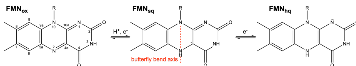
Scheme 2 The physiologically relevant oxidation states of FMN in NrdI. The red dashed line marks the virtual axis between N5 and N10. The ribityl phosphate group is denoted as R.
