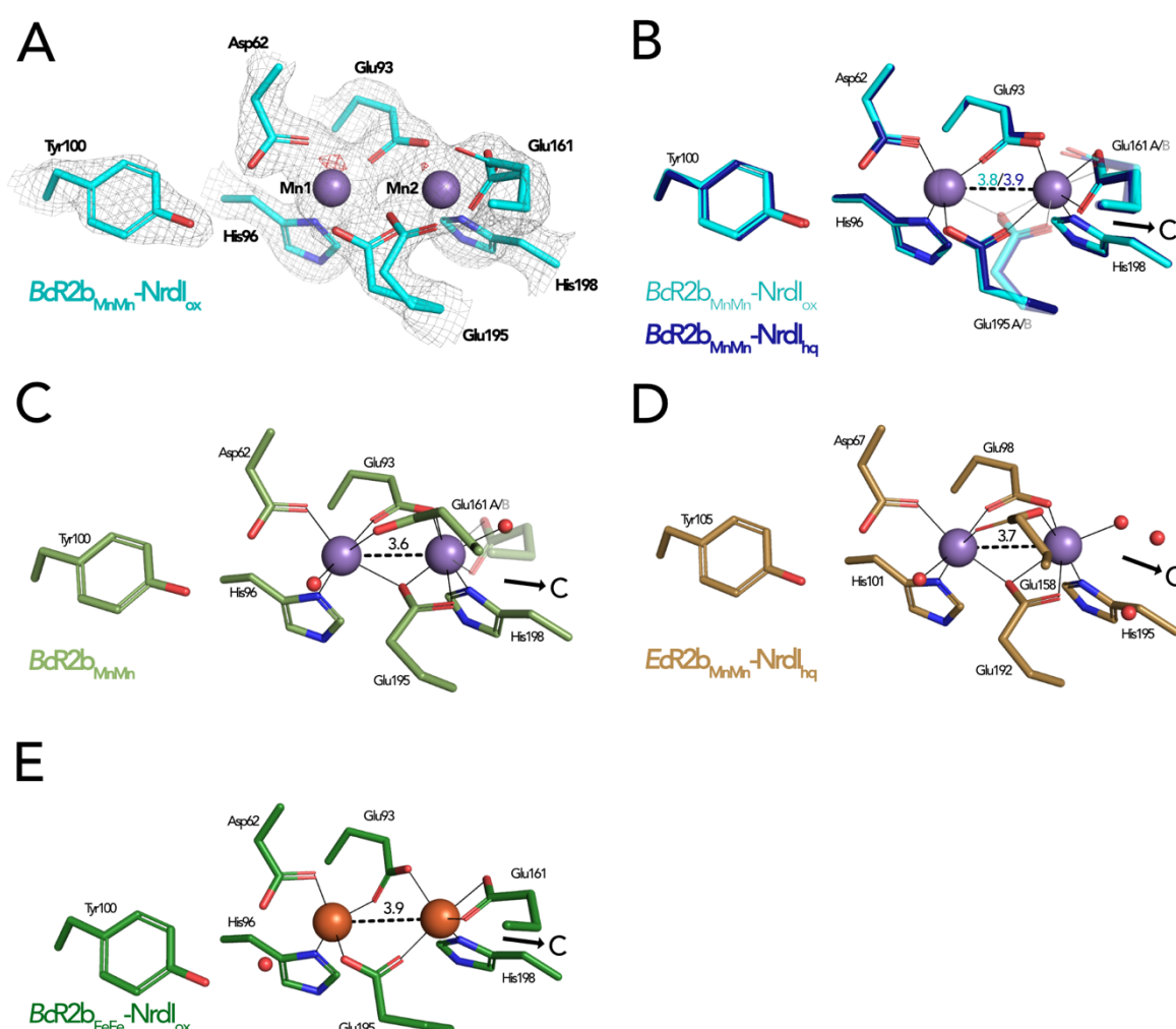
Figure 4 Comparison of active site architecture in different R2b structures including the radical harbouring tyrosine. Manganese ions are shown as purple, iron ions as orange and waters as red spheres. The direction of the connecting channel between R2b and NrdI is indicated by a black arrow and “C”. A) BcR2b MnMn -NrdI ox active site. The 2Fo-Fc map is contoured at 2 \sigma shown as grey mesh and Fo-Fc is contoured at 4 \sigma with negative density
