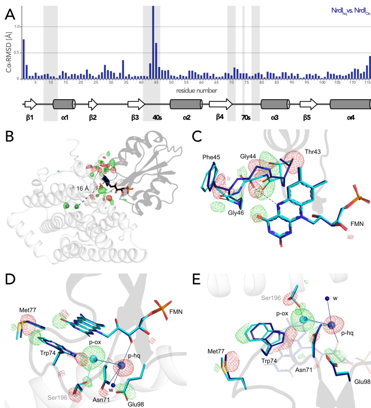
Figure 3 FMN environment in the oxidized and hydroquinone BcR2b-NrdI. A) Structural alignment of NrdI in BcR2b MnMn -NrdI ox compared to BcR2b MnMn -NrdI hq . C \alpha -RMSD in Å are shown for each residue of NrdI between the two models. The secondary structure assignment corresponding to the residues of NrdI is represented in the cartoon below. NrdI interactions with FMN are marked with light grey background B) Fo(ox)-Fo(hq) map contoured at 4.5 \sigma for the BcR2b-NrdI complex with positive density in green and negative density in red. FMN are shown in sticks, manganese ions as purple spheres, R2b as transparent cartoon in white and NrdI in transparent black. Differences between both datasets cluster around the FMN at the R2b/NrdI interface. The distance between metal site and FMN is around 16 Å, marked with a dashed line. C) + D) + E) Close-ups of the
