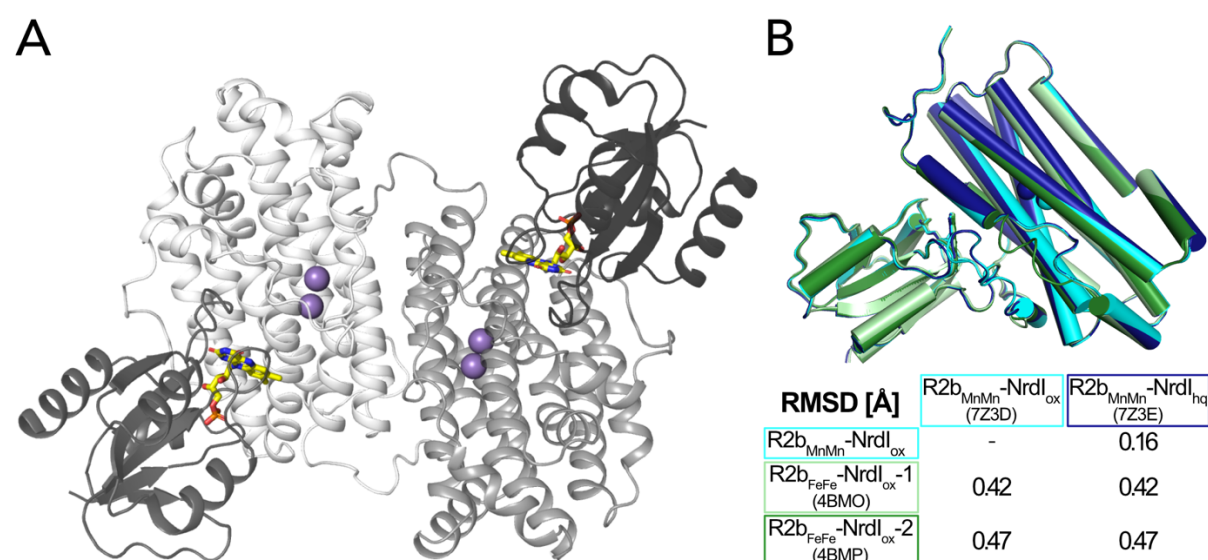
Figure 1 A) Structure of the Bc R2b-NrdI complex (PDB ID: 7Z3D). In each 1:1 R2b-NrdI dimer, R2b and NrdI are coloured in lighter and darker grey, respectively. The second dimer is generated by crystal symmetry. Manganese ions are represented as purple spheres and FMN as yellow sticks at the R2b-NrdI interface. B) Superimposition of all structures of the Bc R2b-NrdI dimer with their corresponding C \alpha RMSD in the table. Individual structures are colour coded identically in the figure and the table.
