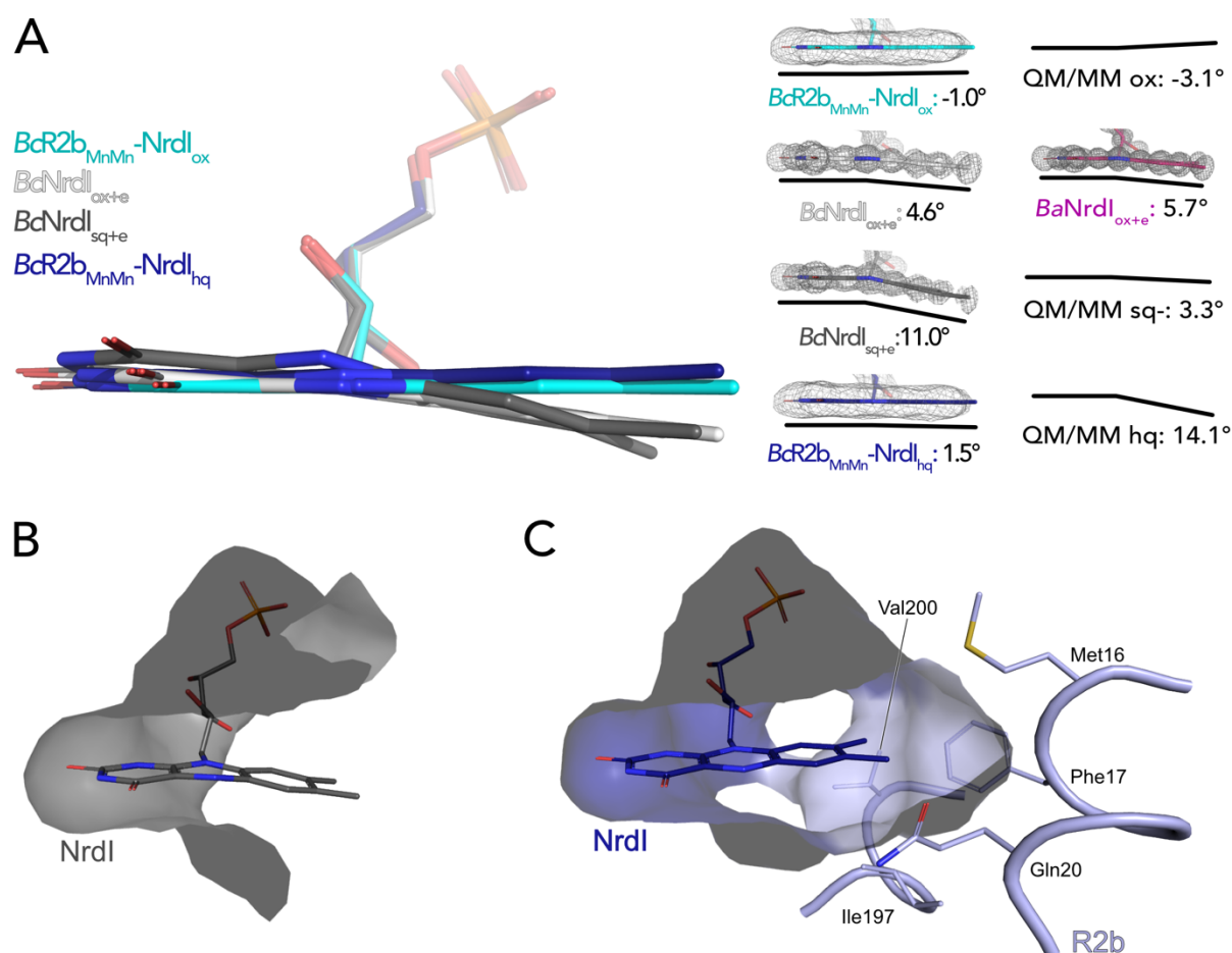
Figure 2 The butterfly bending conformations of FMN in different redox states. A) Left: Overlay of FMN cofactors of B. cereus NrdI in different crystal structures; Right: FMN cofactors in BcNrdI and BaNrdI with 2Fo-Fc maps contoured at 2 \sigma . Additionally, the theoretical calculated butterfly bend angles of FMN bound to BcNrdI are shown (Røhr et al., 2010). Dark blue: BcR2b MnMn -NrdI hq , cyan: BcR2b MnMn -NrdI ox , grey: BcNrdI sq+e (PDB ID: 2X2P), white: BcNrdI ox+e (PDB ID: 2X2O), pink: BaNrdI ox+e (PDB ID: 2XOD). B) The benzene ring of FMN in BcNrdI sq+e (PDB ID: 2X2P) is solvent exposed. C) In BcR2b MnMn -NrdI hq the FMN binding pocket is closed by residues contributed by R2b. Relevant residues are shown in sticks. The surface of the FMN binding pocket in NrdI in panels B) and C) is shown in grey.
