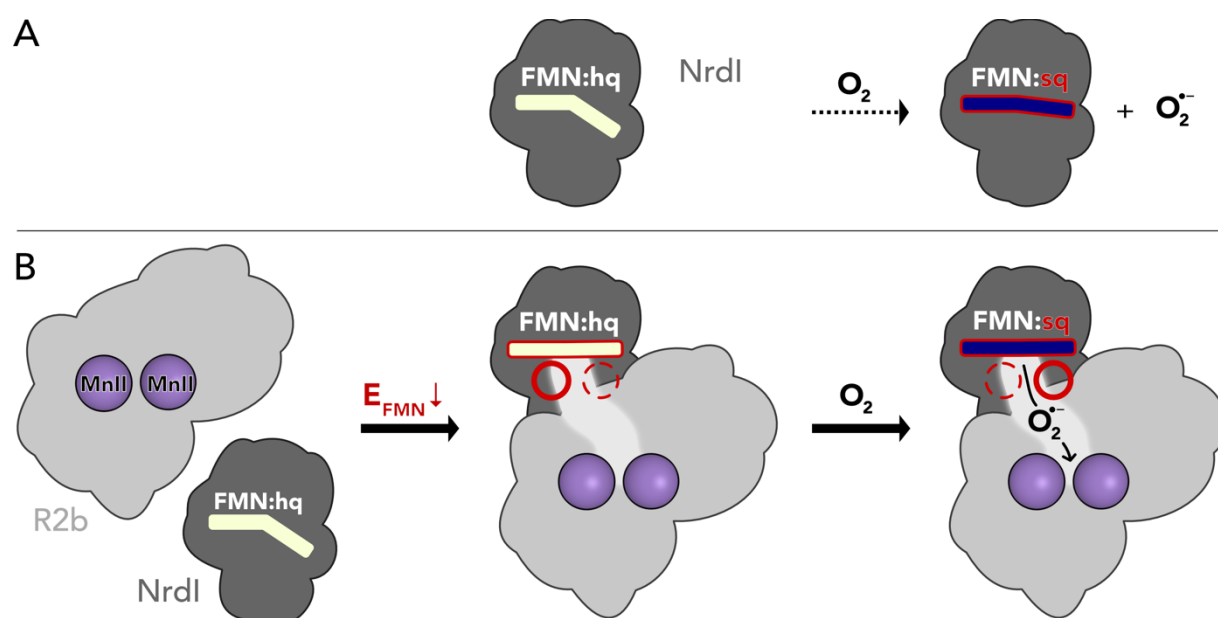
Scheme 3 Proposed mechanism for the assembly of the R2b-NrdI complex. A) Free NrdI hq and molecular oxygen react slowly to produce superoxide and NrdI sq . B) R2b and NrdI form a complex which imposes strain on the FMN bend and lowers its redox potential to favour oxygen reduction. The complex formation also generates a redox
