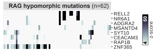
Figure 5 – Figure Supplement 1. A) PhIP-Seq has low detection sensitivity for known antigens USH1C and ANKS4B, but those patients with positive signal exhibit the previously reported coupled signal for both antigens. B) Additional, shared putative antigens within the cohort of RAG1/2-deficient patients (n=62).
