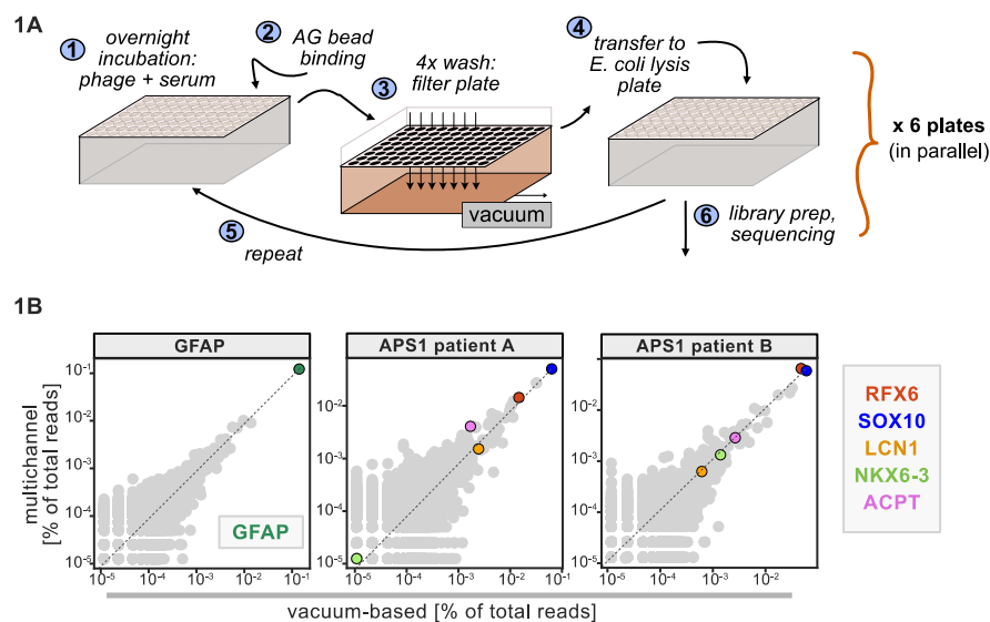
Figure 1. Advantages of and considerations motivating scaled PhIP-Seq. A) Schematic of vacuum-based scaled PhIP-Seq protocol, allowing for parallelized batches of 600-800 samples. B) Comparison of moderate-throughput multichannel protocol data to high-throughput vacuum-based protocol data, with axes showing normalized read percentages. Controls include a commercial polyclonal anti-GFAP antibody (left), APS1 patient A with known and validated autoantibodies RFX6, SOX10, ACPT and LCN1 (center), and APS1 patient B with the same known and validated autoantibodies as well as NKX6-3.
