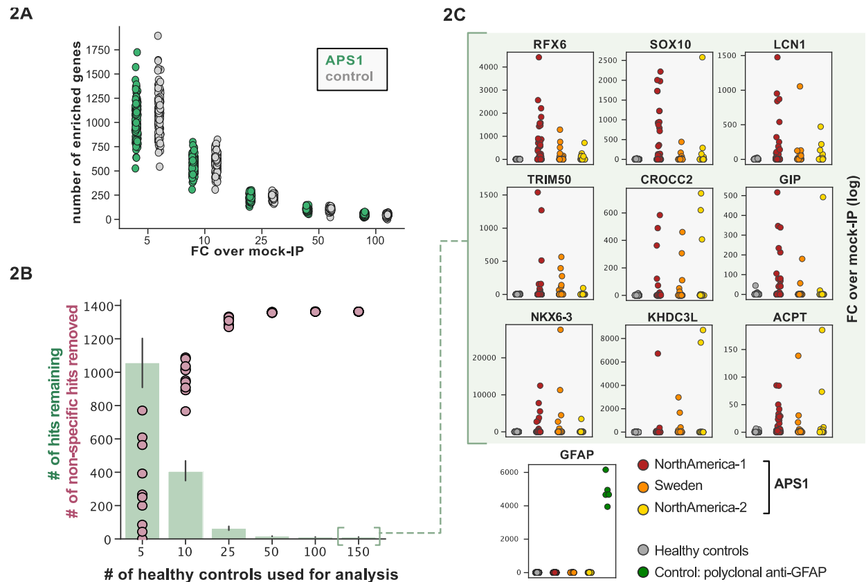
Figure 2. Application of scaled PhIP-Seq to expanded APS1 and healthy control cohorts. A) Number of hits per sample reaching 5, 10, 25, 50, and 100-fold enrichment relative to mock-IP samples. Each dot represents a single APS1 patient (green) or non-APS1 control (grey). B) When looking for disease-specific hits, increasing the number of healthy controls results in fewer apparent hits and is therefore critical. Shared hits are defined as gene-level signal (>10-fold change over mock-IP) which is shared among 10% of APS1 samples (n=128), present in fewer than 2% of healthy controls, and with at least 1 APS1 sample with a high signal (FC of 50<). Random downsampling was performed 10 times for each healthy control bin. C) 9 gene-level hits are present in 10%< of a combined 3-group APS1 cohort. North-America-1, n = 62; Sweden, n = 40; North-America-2, n = 26. Anti-GFAP control antibody (n=5) indicates that results are consistent across plates and exhibit no well-to-well contamination.
