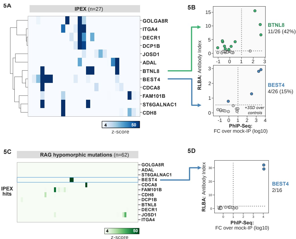
Figure 5. PhIP-Seq screening in IPEX and RAG1/2 deficiency reveals novel, intestinally expressed autoantigens BEST4 and BTNL8. A) PhIP-Seq heatmap of most frequent shared antigens among IPEX, with color indicating z-score relative to a cohort of non-IPEX controls. B) Radioligand binding assay for BTNL8 reveals additional anti-BTNL8 positive IPEX patients (top). Radioligand binding assay for BEST4 autoantibodies correlates well with PhIP-Seq data (bottom). C) PhIP-Seq screen of patients with hypomorphic mutations in RAG1/2 reveals 2 patients with anti-BEST4 signal. D) Orthogonal radioligand binding assay validation of anti-BEST4 antibodies in both PhIP-Seq anti-BEST4 positive patients.
