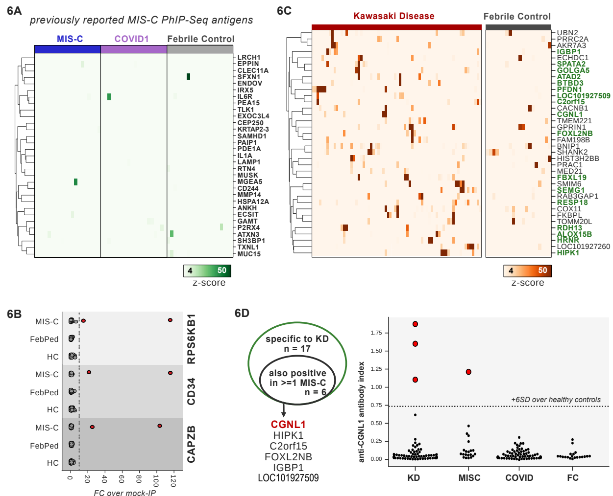
Figure 6. PhIP-Seq screening of MIS-C and KD cohorts. A) Heatmap of signal for putative hits from Gruber et al. 2020, among MIS-C, adult COVID19 controls, and pediatric febrile controls (each n=20). B) Only rare, shared PhIP-Seq signals were found among n=20 MIS-C patients. C) Heatmap of putative antigens in a cohort of n = 70 KD patients. Hits that are specific to KD, and are not found among n=20 febrile controls, are highlighted in green. D) A small number of rare putative antigens are shared between KD and MIS-C (left), with radioligand binding assay confirmation of antibody reactivity to whole protein form of CGNL1 in 3 KD patients and 1 MIS-C patient (right).
