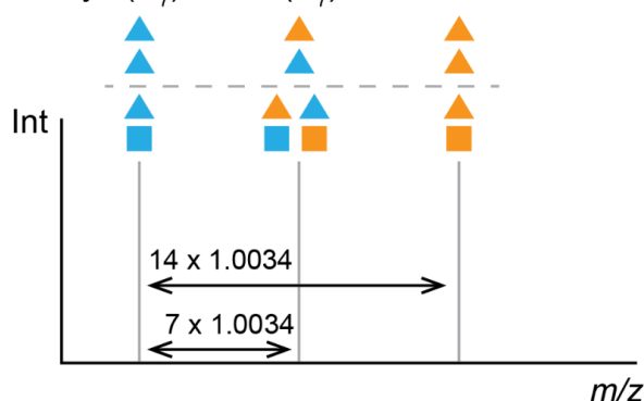
Figure 1 Examples for m/z-patterns produced from mixtures of unlabeled and fully- ^{13}\text{C} labeled molecules. (a) Adenosine diphosphate (ADP), cystine (Cys), and carnitine (Car) present in their fully ^{13}\text{C} labeled and unlabeled form within the same sample. (b) A molecule containing 10 carbon atoms. (c) m/z-pattern of a heterodimer of a \text{C}_{10} and a \text{C}_7 molecule. (d) m/z-pattern of a dimer of two \text{C}_7 molecules. (e) m/z-pattern of a trimer of three \text{C}_7 molecules
