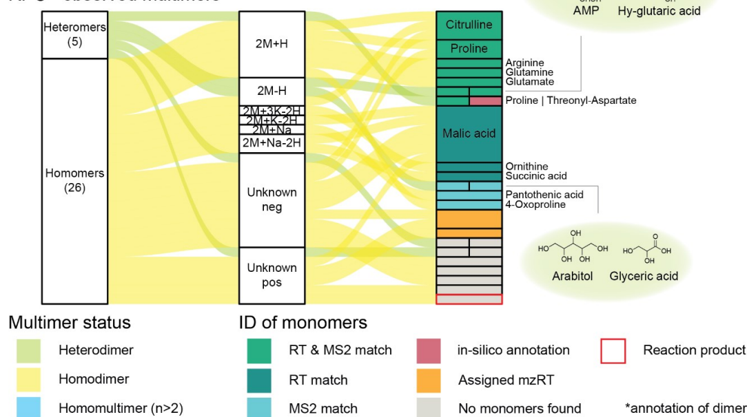
Figure 3 plot of monomer-multimer relationships. (left box) Hetero- and homomers detected after RPC and HILIC analysis. (middle box) Observed multimeric adducts. (right box) Associated PCC-groups with monomer annotation and annotation source.
