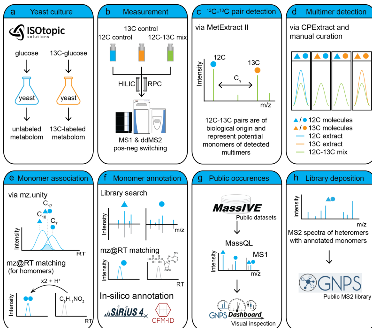
Figure 2 Individual steps of the workflow. (a) Yeast culture extracts were obtained from Isotopic Solutions. (b) 12C13C mixes and controls were analyzed via RPC and HILIC using MS1 and MS2. (c) Biological metabolites were detected as 12C13C pairs. (d) Multimers were detected via characteristic patterns within (see Figure 1) across samples. (e) Monomers were associated with multimers via mz.unify and RT matching to analytical standards. (f) Monomers were annotated via MS2 library searches, RT matching to analytical standards, and in-silico annotation. (g) Occurrences of multimers in public datasets were searched via MassQL and inspected via the GNPS dashboard. (h) MS2 spectra of detected multimers were deposited in the GNPS library for public use.
