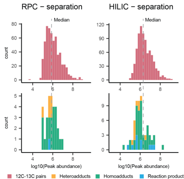
Figure 4 Histograms of peak abundance distributions. Peak abundance distributions for metabolites (12C13C pairs) and multimers colored by their origin for RPC and HILIC. The dashed line indicates the medians for metabolites of both separations.
