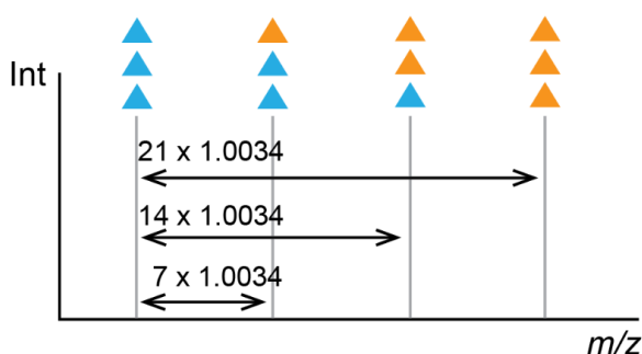
Figure 1 Examples for m/z-patterns produced from mixtures of unlabeled and fully- ^{13}\text{C} labeled molecules. (a) Adenosine diphosphate (ADP), cystine (Cys), and carnitine (Car) present in their fully ^{13}\text{C} labeled and unlabeled form within the same sample. (b) A molecule containing 10 carbon atoms. (c) m/z-pattern of a heterodimer of a \text{C}_{10} and a \text{C}_7 molecule. (d) m/z-pattern of a dimer of two \text{C}_7 molecules. (e) m/z-pattern of a trimer of three \text{C}_7 molecules
