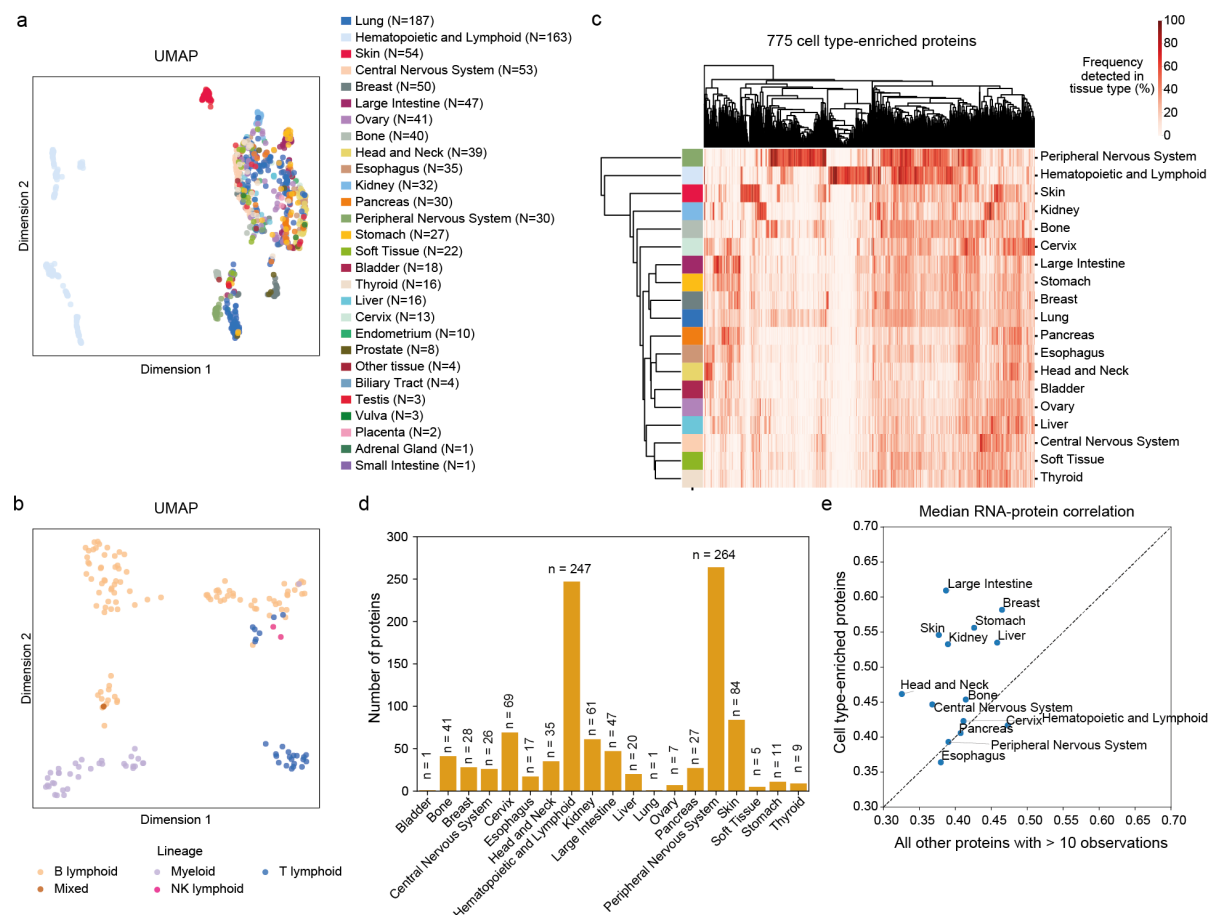
Figure 2. Distinct proteomic profiles according to cell type. a , Proteomic data dimensionality reduction by UMAP, with cell lines colored by tissue. b , UMAP of hematopoietic and lymphoid cell lines colored by cell lineage. c , Heatmap of the frequency of cell type-enriched proteins observed within each tissue. Tissues and proteins are clustered on the vertical and horizontal axes, respectively. d , Number of cell type-enriched proteins identified in each tissue type represented by more than 10 cell lines. e , Median RNA-protein correlation of cell type-enriched proteins against all other proteins with more than 10 observations in that tissue type. Only tissues with at least 10 cell type-specific proteins are shown.
