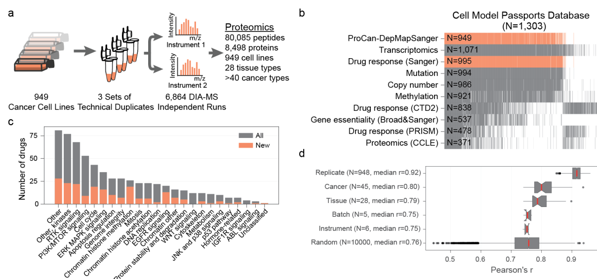
Figure 1. A pan-cancer proteomic map of 949 human cancer cell lines. a , Methodology overview for pan-cancer characterization of 949 human cell lines using a DIA-MS workflow. b , Proteomic measurements were integrated with independent molecular and phenotypic
