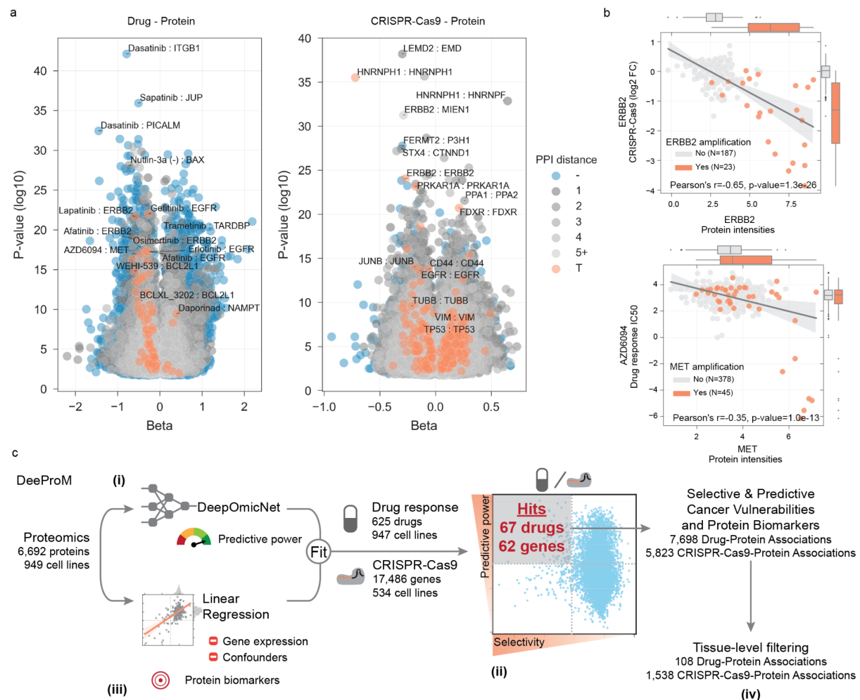
Figure 4. DeeProM identifies protein biomarkers for cancer vulnerabilities. a, Significant linear regression associations ( FDR < 10\% ) between protein measurements and drug responses (left panel) and protein measurements and CRISPR-Cas9 gene essentiality scores (right panel). Each association is represented using the linear regression effect size (beta) and its statistical significance (log-ratio test), and colored according to the distance between the target of the drug or CRISPR-Cas9 and the associated protein in a protein-protein interaction network assembled from STRING. T denotes the associated protein is either a canonical target of the drug or the CRISPR-Cas9 reagents; numbers represent the minimal number of interactions separating the drug or CRISPR-Cas9 targets to the associated proteins; and the symbol '-' denotes associations for which no path was found. Representative examples are labeled. b, Representative top-ranked CRISPR-Cas9-protein and drug-protein associations. Upper panel shows ERBB2 protein intensities associated with CRISPR-Cas9 gene essentiality, where cell lines with ERBB2 amplifications are highlighted in orange. Lower panel shows the association between AZD6094 MET inhibitor and MET protein intensities, where MET amplified cell lines are highlighted in orange. c, Overview of the DeeProM workflow: (i) deep learning models of
