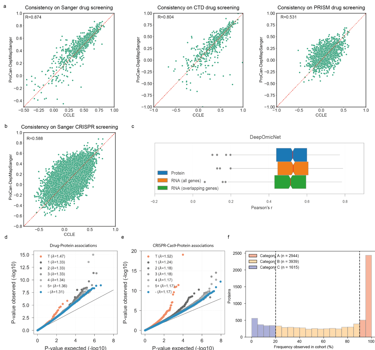
Figure S5. Predictive power benchmarks and comparisons. a , Comparison of DeepOmicNet mean predictive power across three independent drug response datasets, trained using the ProCan-DepMapSanger and the CCLE proteomic dataset. b , Similar to a , models trained to predict CRISPR-Cas9 gene essentiality profiles. c , Comparison of the predictive power of the DeepOmicNet model trained using the ProCan-DepMapSanger dataset and RNA expression data, both for all genes or for only genes that have their corresponding proteins quantified (overlapping genes). d , Drug responses (drug-protein) and e , CRISPR-Cas9 gene essentiality (CRISPR-Cas9-protein) associations, identified with linear regression models without taking gene expression as covariates. See Figure 7c-d for a general description of the plot. f , Histogram showing the distribution of the frequency of proteins detected in each of the cell lines in the cohort, with Category A, B and C proteins indicated. The dashed vertical lines indicate the frequency thresholds for defining the categories.
