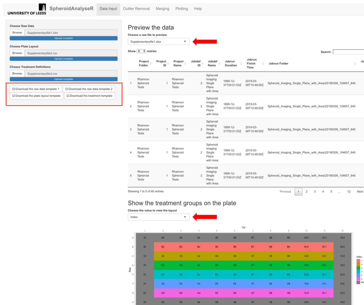
Figure 1. The Data Input tab once raw data has been uploaded. Template files are available to download (see red rectangle). A raw file (Supplementaryfile1), plate layout (Supplementaryfile2) and treatment file (Supplementaryfile3) have been uploaded. A preview of the raw data is shown in the main panel, and a map of the plate coloured by treatment index is displayed underneath. Red arrows show the dropdown menus to select a different file to view, and to choose a value to view the layout for.
