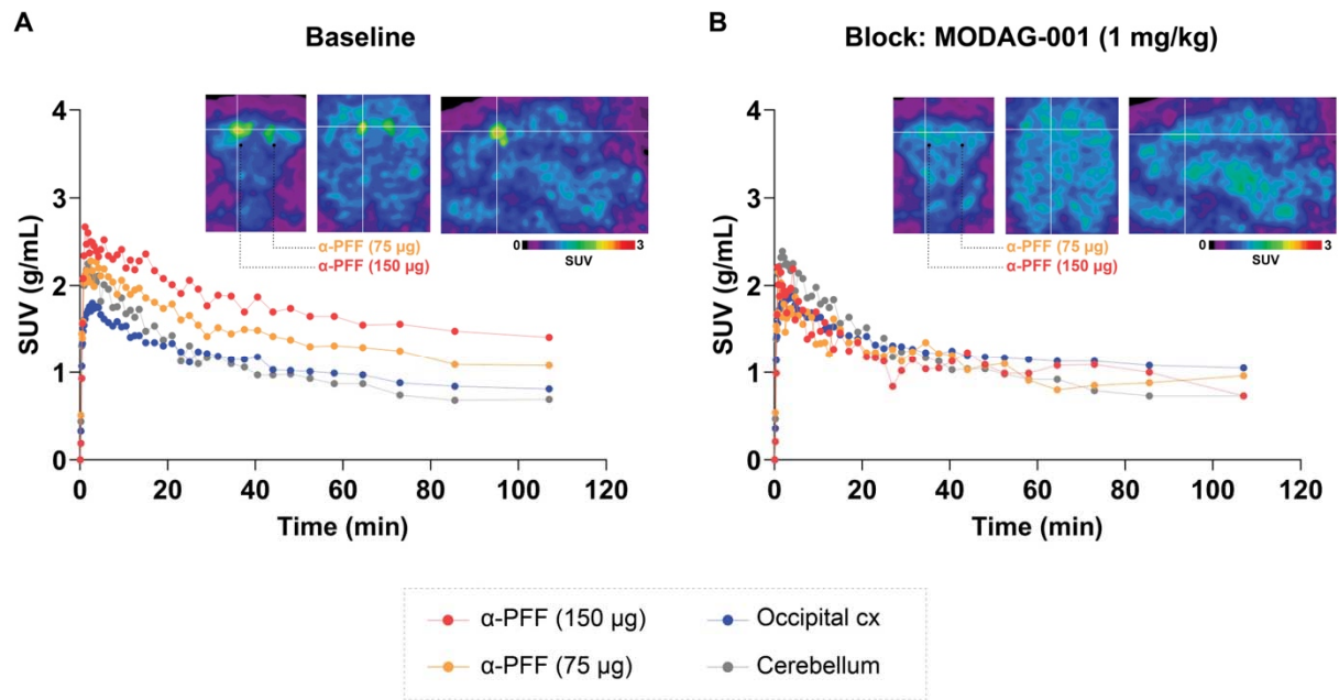
Figure 2. (d 3 )-[ 11 C]MODAG-001 baseline and block. TACs and SUV scaled PET images A) (d 3 )-[ 11 C]MODAG-001 baseline and B) (d 3 )-[ 11 C]MODAG-001+ MODAG-001 (1 mg/kg) block scan from a pig with 150 µg and 75 µg α-PFF.
