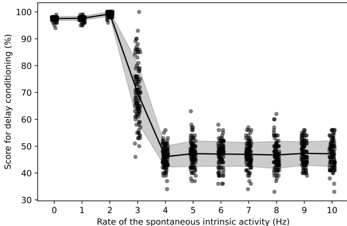
Figure 5. Effect of spontaneous intrinsic activity on the performance during the delay conditioning on the cognitive level .
