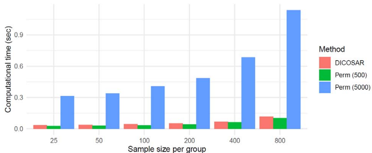
Figure 5. The computational time of DICOSAR for a single test for the equality of the PCCs of a pair of variables between two groups and its comparison with that of the permutation methods. The benchmark is computed based on the average computational time across 20 randomly generated data sets. Perm (500) & Perm (5000): the pooled residual permutation method with 500 and 5000 replicates, respectively.
