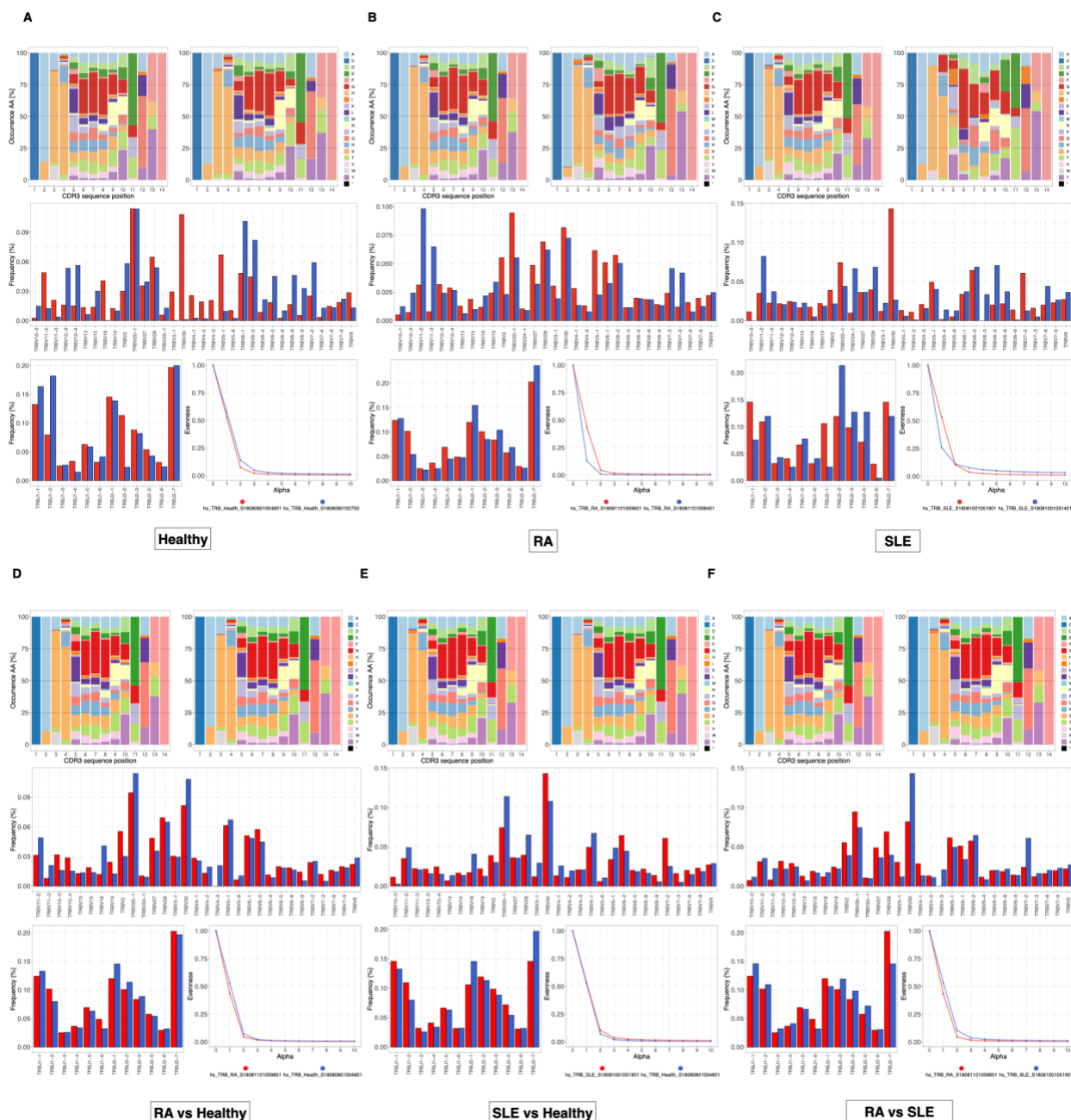
Supplementary Figure 10 | Within and cross-immune state similarity of repertoires is high (Healthy, RA, SLE) for the PIRD human T-cell dataset (Zhang et al.,2019). The amino acid frequency (first row), VJ usage (middle row, bottom left) and evenness (bottom right) compared (A–C) between the most (left amino acid plot, red bars, and lines ) and least (right amino acid plot, blue bars, and lines) locally similar repertoires of each immune state. (D–F) between the most locally similar repertoires of each immune state pair.
