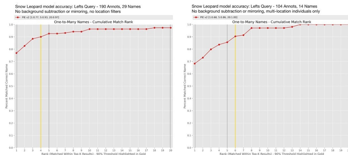
Fig 5. Accuracy on a PIE model without background subtraction or L/R mirroring. Left is without location filtering; right is only multi-location individuals that moved between trapping stations.
