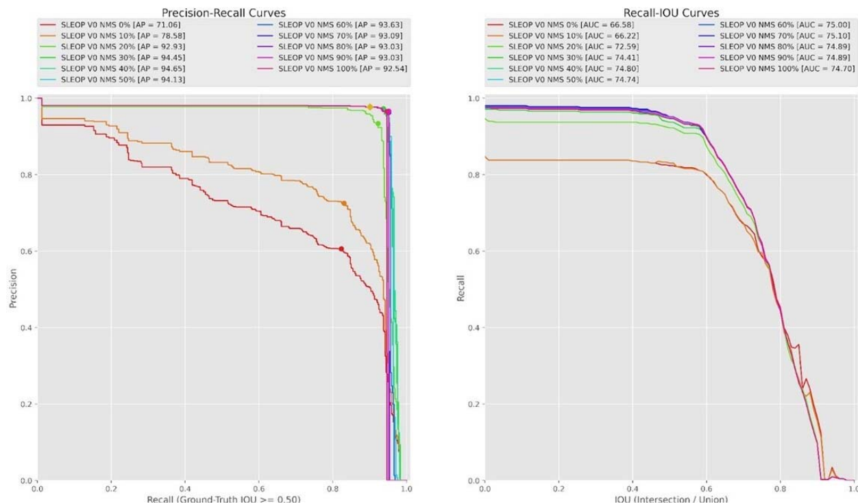
Fig 3. The detector Precision-Recall curves for snow leopards.
