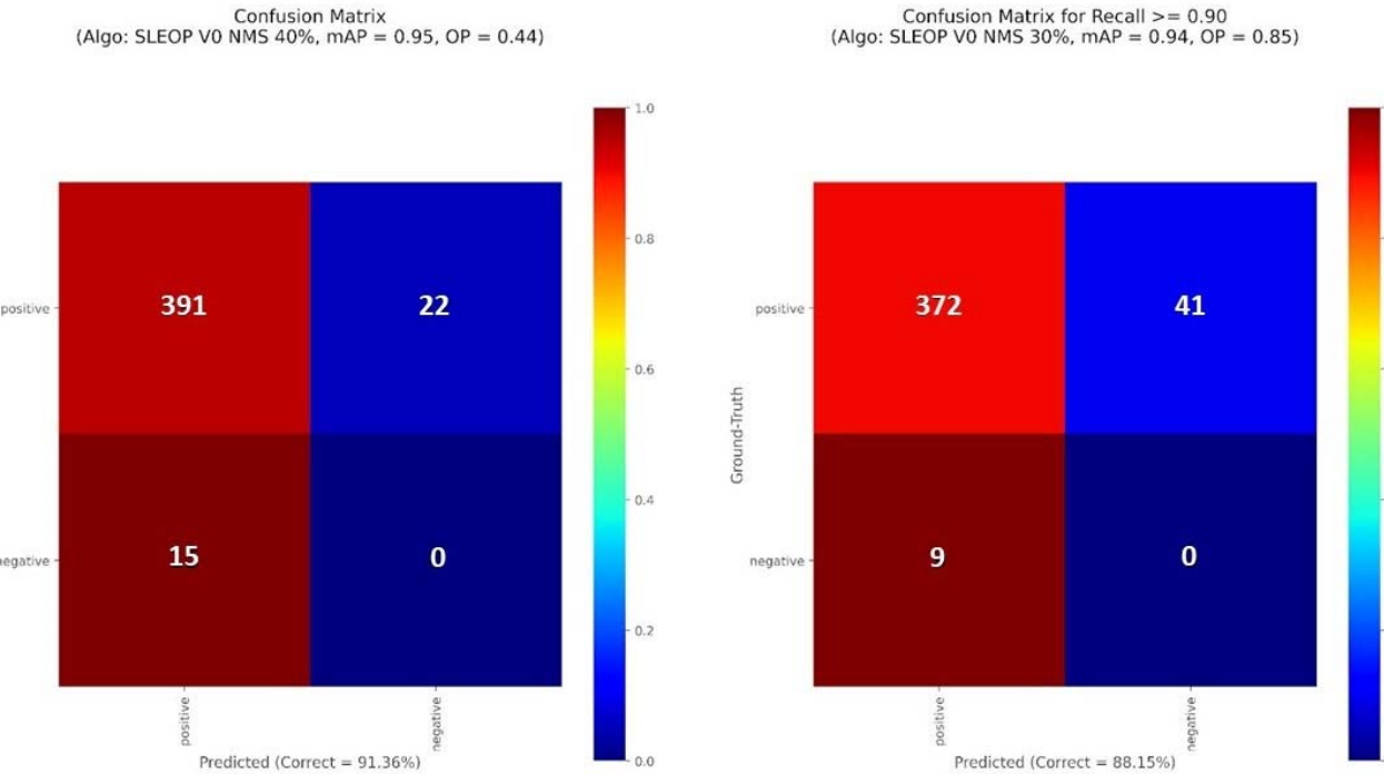
Fig 4. Confusion matrices for the best-colored point (left) and the yellow diamond (right) from the Precision-Recall performance curves (Fig. 2). False negatives occur when not detecting a snow leopard when one is present in the image, and false positives are spurious detections when no snow leopard is present in the image, such that a bounding box is generated where there is no snow leopard within it.
