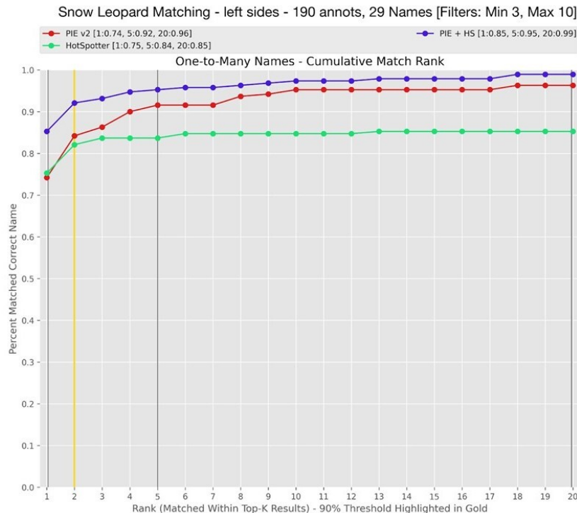
Fig 7. Accuracy plot of the deployed matching algorithm. Left-side annotations of individuals contain at least three left-side photos. Right-side performance is roughly equivalent (this model mirrors left-side photos, so every animal it sees is from a right-side perspective, but queries are pre-filtered by viewpoint not to compare lefts and rights).
