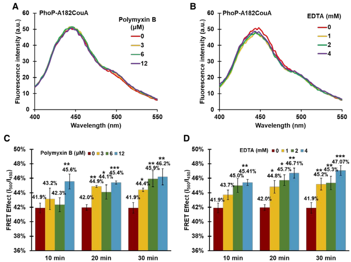
Figure 6. Comparison of PhoP activities in response to \text{Mg}^{2+} depletion and polymyxin B treatment. (A & B) Fluorescence spectra of BL21 (DE3) cells expressing PhoP-A182CouA (AY3709) treated by polymyxin B (A), or EDTA (B). (C & D) FRET effect of the CouA-SYTO 9 pair in the designated assay mixtures. Data are the mean of three biological repeats and are expressed as mean \pm SD. *, P < 0.05 ; **, P < 0.01 ; ***, P < 0.001 (based on Student's t test).
