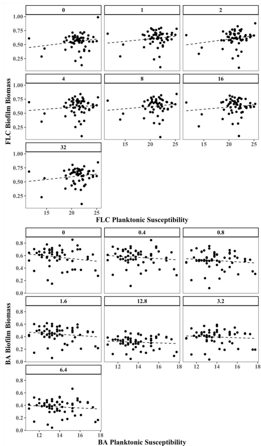
Supplementary Figure 1 Association of planktonic susceptibility and biofilm biomass of C. albicans isolates. There is no association between planktonic susceptibility and biomass of the biofilms for both FLC and BA (linear mixed-effect model).
