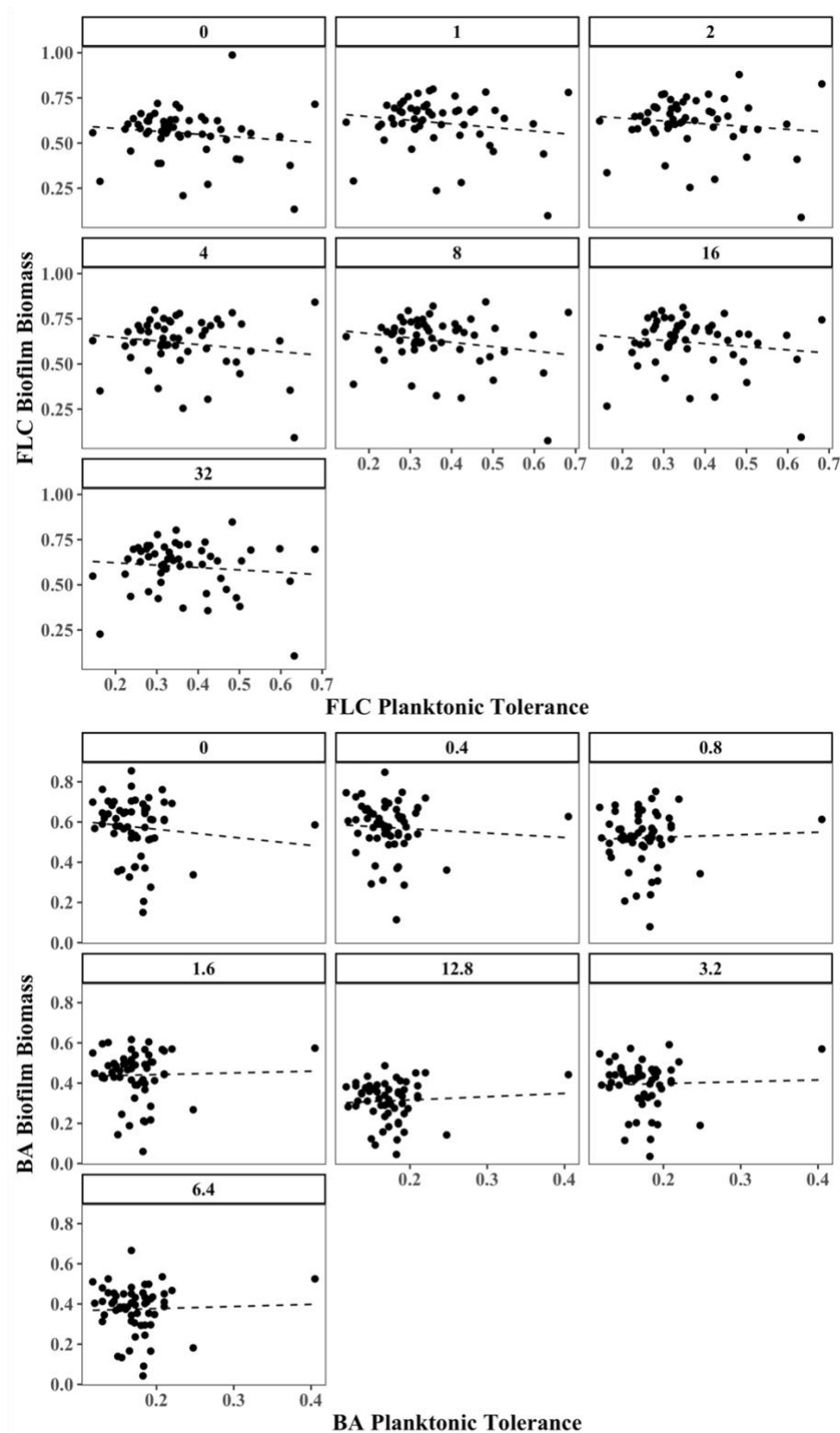
535 Supplementary Figure 3 Association of planktonic tolerance and biofilm biomass of C. albicans isolates. There is no association between planktonic tolerance and biomass of the biofilms for both FLC and BA (linear mixed-effect model).
