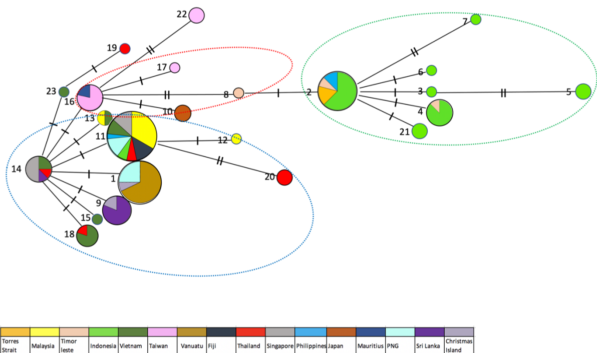
Figure 2. Haplotype network for COI. Each coloured node represents an observed haplotype with circle size indicating the number of individuals with each numbered haplotype and the slash along the connecting lines indicating the number of nucleotide differences.
