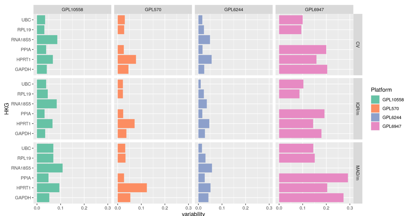
Figure 3. Variability levels for the classic housekeeping group evaluated in Hsa. For each of the housekeeping genes, the variability level found in the selected microarray platforms with the three statistical approaches (C.V., IQR/median and MAD/median) is described on the X-axis.
