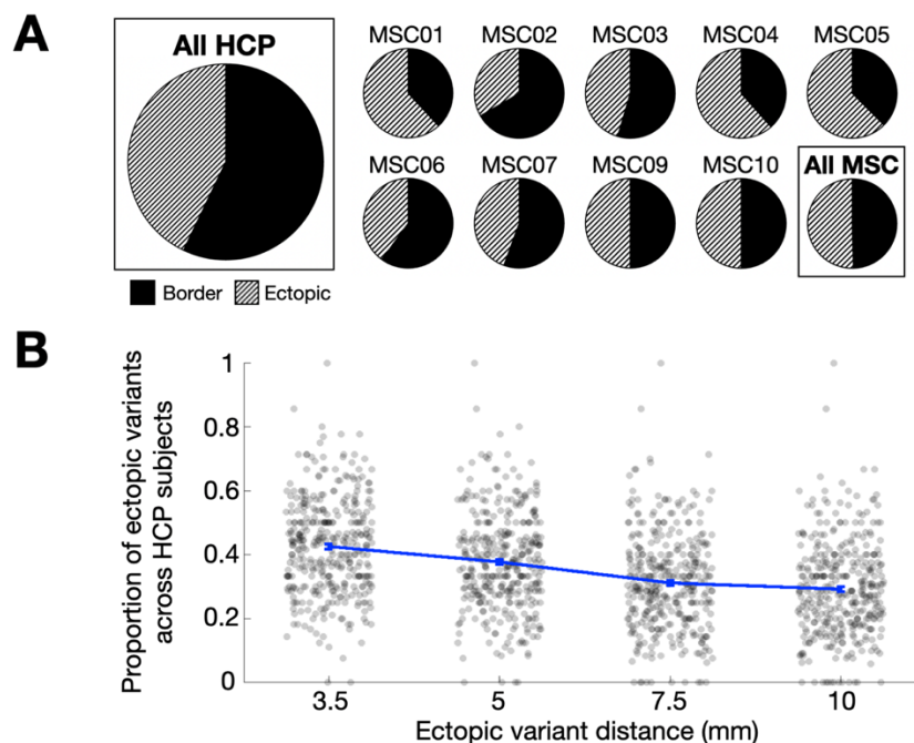
Fig. 2: Prevalence of border and ectopic variants across individuals. (A) The panel displays the proportion of border and ectopic variants across all subjects in the HCP dataset (far left), and within subjects in the MSC dataset (two rows on right). Both ectopic variants and border variants were consistently identified in almost all individuals in both the HCP and the MSC datasets. (B) Proportions of ectopic variants at other distances (error bars represent
