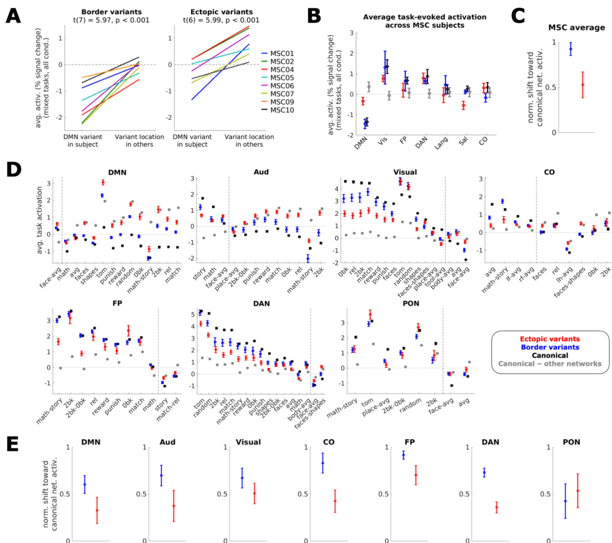
Fig. 5: Task-evoked activation of variant locations in the MSC and HCP. (A) Average activation in the MSC of DMN-assigned variants in an individual vs. average activation in that location in all other individuals for border (left) and ectopic (right) variants; 8 of 9 subjects with a border DMN variant and 7 of 9 subjects with an ectopic DMN variant were included. Different colors represent different MSC participants. Both border and ectopic variants exhibited functional activation shifted from the typical responses of their location toward the response expected based on their network associations. Similar results were seen with our secondary method of border/ectopic variant classification (Supp. Fig. 16). (B) Average activation ( z ) across all task conditions in a set of mixed-design tasks from the MSC for variants (red = ectopic, blue = border shift), canonical locations of the listed network (black), or canonical locations of other networks (gray). Error bars represent the standard error of the mean across subjects. Data were only included from individuals that had a variant of the given form and network (e.g., a border variant assigned to the DMN). (C) Normalized shift of border (blue) and ectopic (red) variants toward the listed canonical networks. Values represent the average normalized value across the listed networks (calculated as (\text{variant} - \text{other networks}) / (\text{canonical network} - \text{other networks}) ); error bars represent standard error of the mean across networks. (D) Average task activation across HCP subjects. For each network, contrasts were included if the activation in canonical regions of the network was greater than that of other networks by a margin of at least 0.5% signal change. Vertical dashed lines mark the delineation between contrasts where a given canonical network's activation is greater than other networks' activation and contrasts where other networks' activation is greater. Error bars represent standard error of the mean across subjects for a given contrast; see Supp. Table 2 for information on tasks associated
