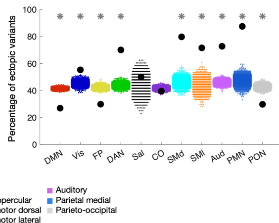
Fig. 4: Network linkages of border and ectopic variants (A) Network distributions of border and ectopic variants in the HCP dataset. Variants of both forms are commonly associated with the DMN, FP, and CO networks, as reported in past work 15 . Similar results were seen in the MSC dataset (Supp. Fig. 13) and using the parcellation-free approach to defining border and ectopic variants (Supp. Fig. 14) (B) Plot depicting permutation testing of the ectopic: border ratio in the HCP dataset. For all networks with the exception of salience and cingulo-opercular, the true proportion of ectopic variants (black dots) was significantly different from permuted proportions (colored dots, 1000 random permutations of shuffled labels) at p < 0.001 (*; FDR corrected for multiple comparisons). DMN, FP, and PON variants were more likely to be border shifts, while sensorimotor, DAN, and PMN variants were more likely to be ectopic. Notably, ectopic variants were commonly found in all systems. See Supp. Fig. 12 for cortical depiction of each listed network.
