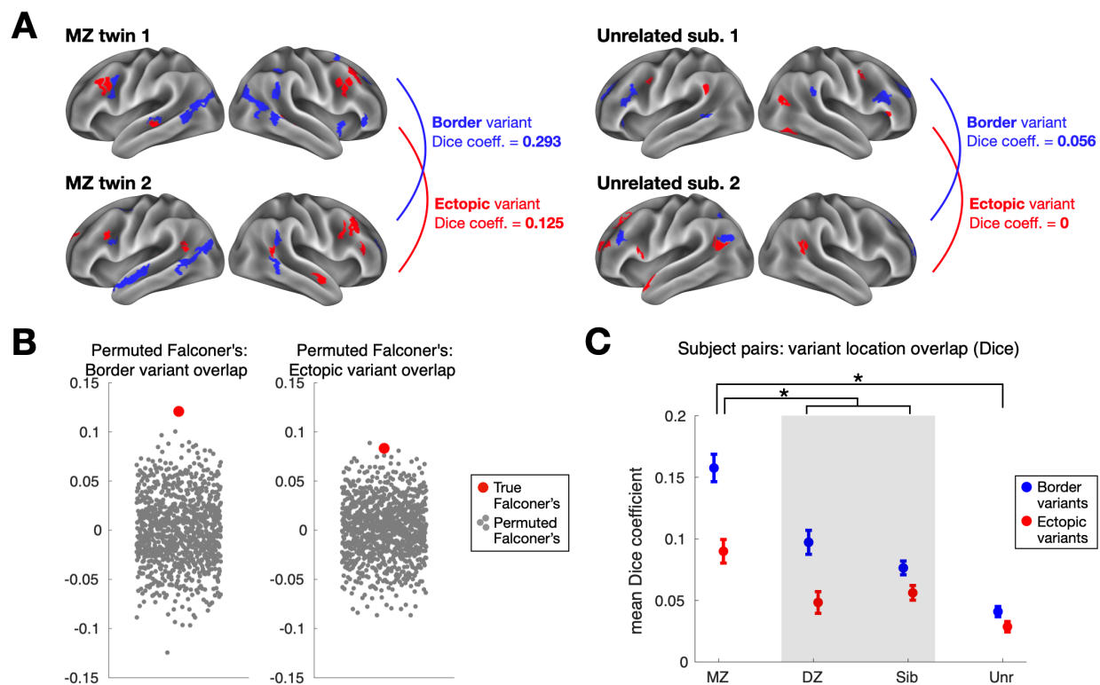
Fig. 6: Estimating the genetic influence of border and ectopic variants across individuals in the HCP dataset. (A) The similarity of border (blue) and ectopic (red) variant locations was measured for monozygotic (MZ) and dizygotic (DZ) twin pairs, siblings, and unrelated individuals. This schematic shows an example pair of MZ twins (left) and unrelated individuals (right). The MZ twins exhibit a greater Dice coefficient of overlap between their border variants (in blue) and ectopic variants (in red) than a pair of unrelated subjects. (B) This observation was confirmed by estimating genetic influence with Falconer's formula, which compares similarity in MZ and DZ twins. Both border and ectopic variants (red dots) exhibited significant similarity ( p < 0.001 and p < 0.002 respectively) relative to a permuted null (gray dots) where MZ and DZ labels were randomly shuffled ( *note, our use of Dice instead of R-values in Falconer's formula does not produce heritability estimates, but does provide a valid way to assess non-zero genetic influence via permutation testing, randomly shuffling MZ and DZ labels ). (C) Average similarity among border and ectopic variants is shown for pairs of HCP participants. For both forms of variants, MZ twins showed the highest similarity, DZ twins and siblings showed intermediate similarity, and unrelated individuals showed the lowest similarity, a pattern consistent with an influence on genetics on variant locations. Bars represent standard error across subject pairs.
