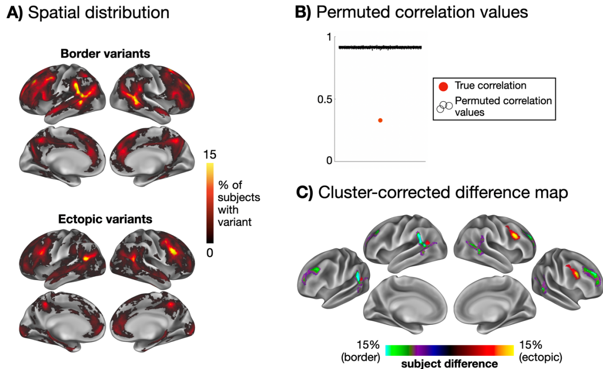
Fig. 3: Spatial distributions of ectopic and border variants. The maps in (A) show the spatial distribution of border variants and ectopic variants, overlapped across participants in the HCP. (B) These two spatial distributions differ significantly more than expected by chance from random permutations. Permuted correlation values are jittered across the x-axis for visualization. (C) A cluster-corrected difference map is shown highlighting regions with a significantly higher occurrence of border variants (green/purple) and ectopic variants (yellow/red; p < 0.05 cluster-corrected for multiple comparisons based on permutation testing). Ectopic variants were more prevalent in the right posterior inferior frontal sulcus and left posterior TPJ regions, while border variants were more prevalent in dorsal and ventral portions of the anterior TPJ and superior rostral frontal regions. See Supp. Fig. 9 for evidence of similar results for ectopic variants at greater distances, Supp. Fig. 10 for similar results using our secondary parcellation-free variant definition method, and Supp. Fig. 11 for border and ectopic overlap maps for each network individually.
