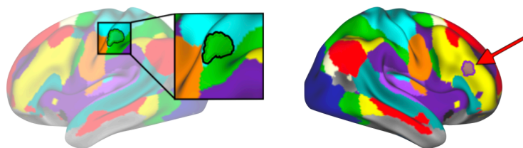
Fig. 1: Variant definition, splitting, and classification as border or ectopic. (A) Following Seitzman et al. 15 , we used spatial correlation to compare the seedmap at a given location between an individual and an independent group average (left) to generate an individual-to-group “similarity map” (middle). This similarity map was thresholded and binarized to identify locations with low similarity to the group (right) that we call “pre-variants” in this work (Note: these were also thresholded to remove small areas and areas of low signal - see Methods ). We then further refined these pre-variants to create homogeneous units for border vs. ectopic variant classification (see Methods and Supp. Fig. 1 for a description of this process). (B) Each variant was classified as either a border shift or an ectopic intrusion based on its edge-to-edge distance from the nearest same-network boundary in the group-average network map. Here, we display an example of a border shift variant (left, green region with black outline) and an ectopic variant (right, purple region with dark outline), overlaid on the group average network map. Distances > 3.5 mm were classified as ectopic; distances < 3.5 mm were classified as border (see Fig. 2B and Supp. Fig. 8 for exploration of additional distance criteria). We also employed a secondary method for defining border and ectopic variants that did not rely on a group-level network parcellation (see description in Methods and Supp. Fig. 2).
