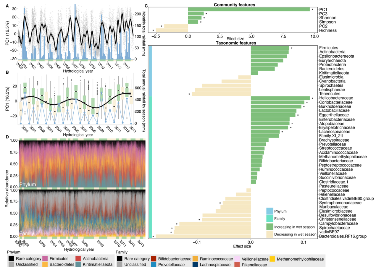
Fig. 2. Baboons show population-wide, cyclical shifts in microbiome community composition across seasons and years. (A) Changes in microbiome PC1 mirror monthly rainfall across all 14 years. The grey points show values of PC1 for each of the 17,265 samples (y-axis) on the dates they were collected (x-axis). The black line and its grey band show the predicted daily trend for PC1 across samples and its 95% simultaneous confidence interval, treating time as a continuous variable from April 21, 2000 to September 19, 2013. Blue bars show monthly rainfall (right-hand y-axis), and the yellow and green bars along the x-axis represent dry and wet seasons, respectively, with the width reflecting the number of months within the focal year with at least 1 mm rainfall. (B) Changes in microbiome PC1 on an annual scale across all 14 years (N = 17,265 samples). The box plots show the distribution of PC1 in wet (green) and dry (yellow) seasons. The black line shows the estimated annual trend for PC1 across all hydrological years, and the blue points show total annual rainfall (right-hand y-axis). (C) The effect of season varies across 52 features of the microbiome, including six community features (top panel) and 46 taxa (bottom panel; 12 phyla: light blue vertical bar; 34 families:
