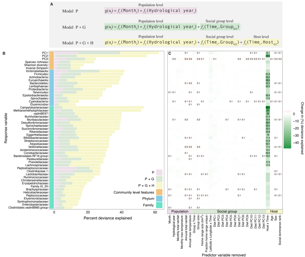
451 452 Fig. 4. Multilevel modeling identifies idiosyncratic microbial dynamics. (A) We fit three 453 hierarchical GAMs to 52 microbiome features measured in 4,277 samples from the 56 best- 454 sampled baboons, all of whom lived in the 5 social groups sampled the longest (between 2002 455 and 2010; median = 72.5 samples per host; minimum = 48 samples; maximum = 164 samples; 456 fig. S3 ). Each model contained successive sets of predictor variables reflecting population-level 457 factors (pink), group-level factors (green) and host-level factors (yellow). The factors at each 458 level are listed at the bottom of panel C and defined in table S5 ). Panel (B) shows, for each 459 microbiome feature (i.e., response variable), the deviance explained by model P and the 460 successive sets of predictor variables added in model P+G and model P+G+H, respectively 461 ( table S6 ; percent deviance is a measure of goodness-of-fit for nonlinear models and is 462 analogous to the unadjusted R^2 for linear models). Panel (C) shows the loss in deviance 463 explained for model P+G+H as we successively removed each predictor variable in turn from
