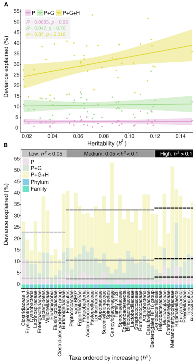
Fig. 5. Microbiome taxon heritability is associated with idiosyncratic dynamics. (A)
