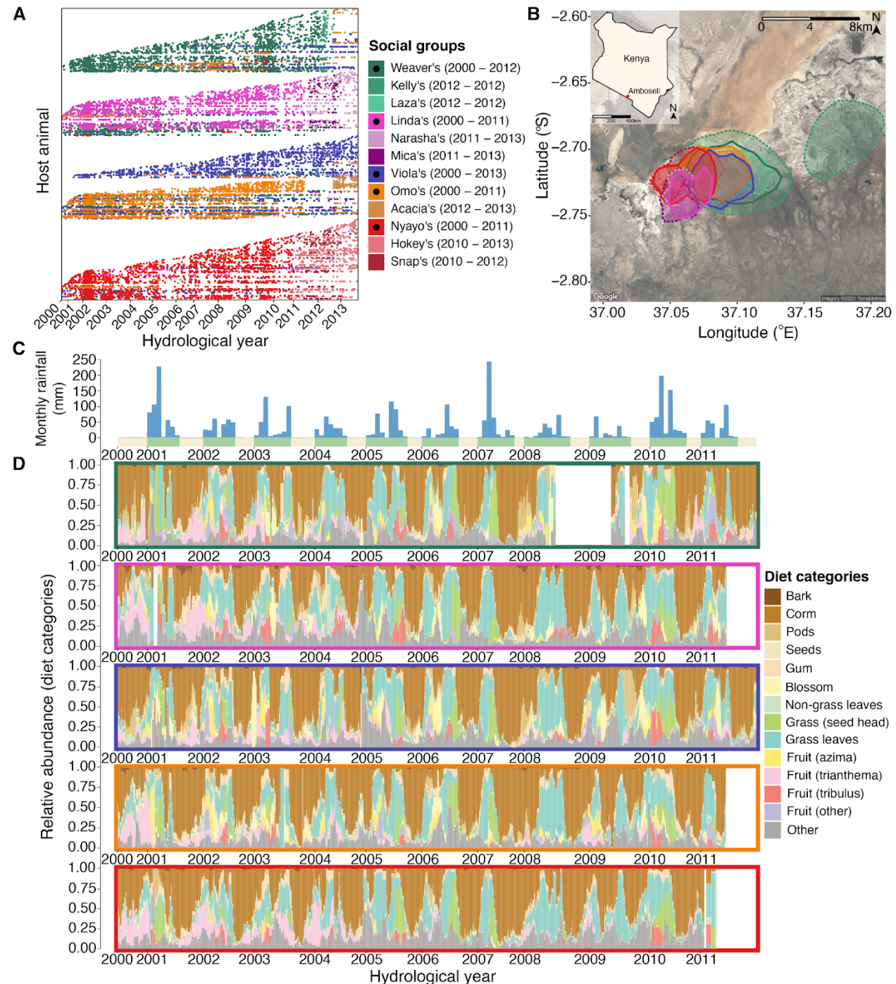
Fig. 1. Baboons in Amboseli experience shared environments at multiple scales. (A) Our microbiota time series consisted of 17,265 16S rRNA gene sequencing gut microbial profiles. Each point represents a microbiota sample, plotted by the date it was collected (x-axis). Each
