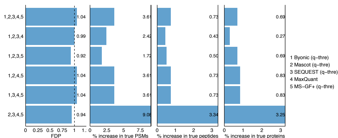
Figure S9 On the proteomics standard dataset, comparison of APIR and individual database search algorithms at the FDR threshold q = 1\% in terms of FDR control and power
