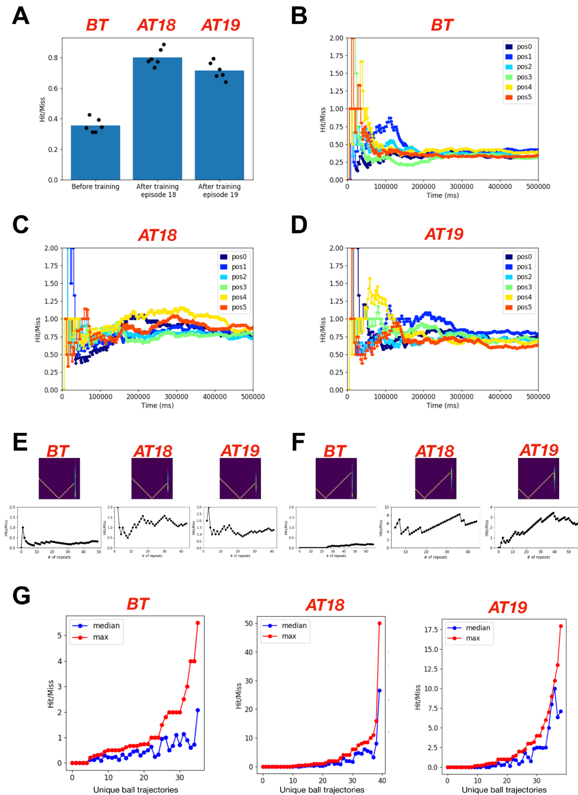
Figure 4. The feedforward spiking neuronal network model sustained its performance after learning. A) The bar plot shows the mean (n=6) performance (Hit/Miss) of the model before training (using initial weights), after training episode 18 and after training episode 19. For each condition, 6 different initial positions of the racket and the ball were used to evaluate and compare the
