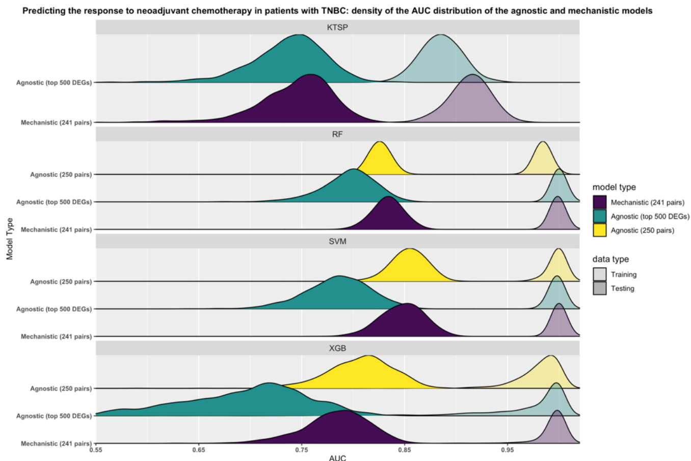
Figure 4. NOTCH-MYC-based models outperform their agnostic counterparts in predicting response to neoadjuvant chemotherapy in patients with triple-negative breast cancer. Models were trained on 1000 bootstraps of the training data (transparent colors) and evaluated on the untouched testing data (solid colors) using the Area Under the ROC curve (AUC) as metric. Mechanistic models were based on the NOTCH-MYC mechanism (241 pairs) (purple) while agnostic models were trained either using the top differentially expressed genes (500 genes) (green) or the corresponding pairwise comparisons (250 pairs) (yellow). Shown are the smoothed density distributions of the AUC values with each panel corresponding to one of the four algorithms used. KTSP: K-top scoring pairs; RF: random forest; SVM: support vector machine; XGB: extreme gradient boosting; DEGs: differentially expressed genes; TNBC: triple-negative breast cancer.
