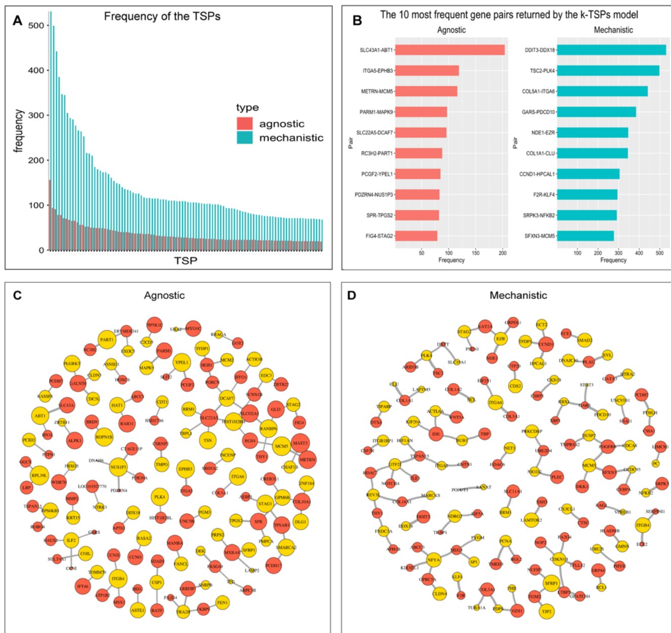
Figure 5. Mechanistic and agnostic k-TSPs signatures for predicting the response to neoadjuvant chemotherapy in patients with triple-negative breast cancer. A) Bar plot showing the frequency of the top 100 agnostic (red) and mechanistic (blue) scoring pairs across the different bootstraps. B) The top 10 most frequent agnostic (red) and mechanistic (blue) pairs sort by their frequency. C-D) Networks of the top 100 agnostic (C) and mechanistic (D) top-scoring pairs. Each pair consists of a gene voting for RD (red) and pCR (yellow). The vertex size corresponds to 2 \times \log_2 of the individual gene frequency across unique pairs while the edge thickness corresponds to the \log_2 of the top scoring pair frequency.
