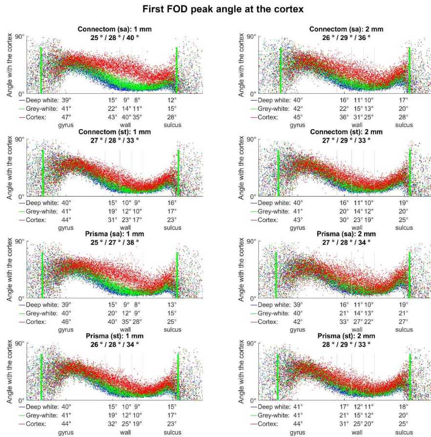
Figure 4: Effect of scanner, acquisition, resampling on the orientation of FODs (calculated for 1 st peak only) in relation to the cortex, depending on the location along the gyral blade. Each plot shows average angle distributions across all subjects, sampled at three depths (green: grey-white interface, blue: 1 mm deep, red: 1 mm superficial). Mean angle is shown under each title (deep white/grey-white/cortex, respectively); same is provided on the x-axis for the five equal-area sectors of the gyral blade. Grey vertical lines illustrate boundaries between the five sections along the gyral blade. Green vertical lines represent 5-95% range used for average angle calculation. Connectom scanner, “state-of-the-art” sequences, smaller voxel data all demonstrate steeper peak rotation from near-parallel to near-perpendicular orientation (from deep white to cortex, respectively) particularly in
