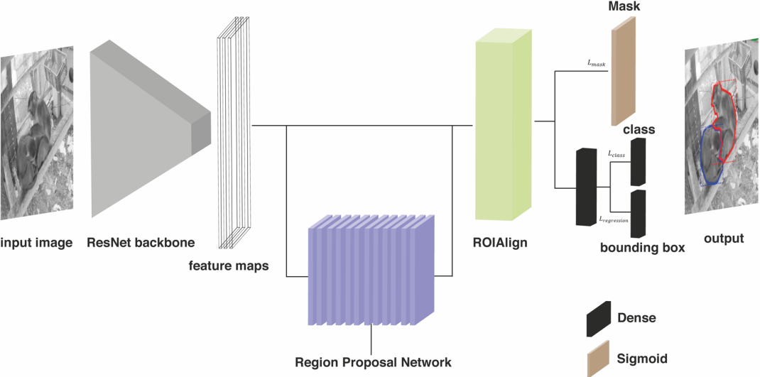
Supplementary Fig. 12 | SIPEC SegNet Architecture.
