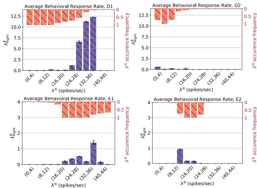
Figure 9: Synthetic Dataset Illustrating the average estimated response rate for each interval of estimated neural activity. Error bars show the standard error. Purple bars show the average behavioural response rates. Orange bars indicate the proportion of trials with the occurrence of each neural response interval. As expected in the RIGHT trials and represented by purple bars, highest behaviour rates are detected in D1 when neural activities approach 40 spikes/s in the (32,36) and (36,40) range. On the other hand, there is little to no activity estimated for D2 which is a leftward preferring integration region. Highest response rates are achieved for when E1 neural activity is in the vicinity of 40 spikes/s (in the (36,40) range) and when the neural activity in E2 is in (12,14) range. These are in agreement with results from Figure 8.
