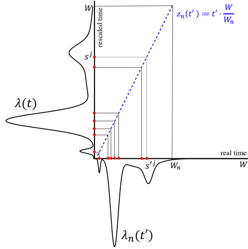
Figure 6: Illustrating the transformation of the Poisson point process in real time \lambda_n(t') , to the rescaled time domain which results a point process with intensity function \lambda(t) . The transformation function z_n(t') = t' \cdot \frac{W}{W_n} performs a one-to-one monotonic mapping of the events in real time ( s'^j ) to the events on the rescaled time axis ( s^j ).
