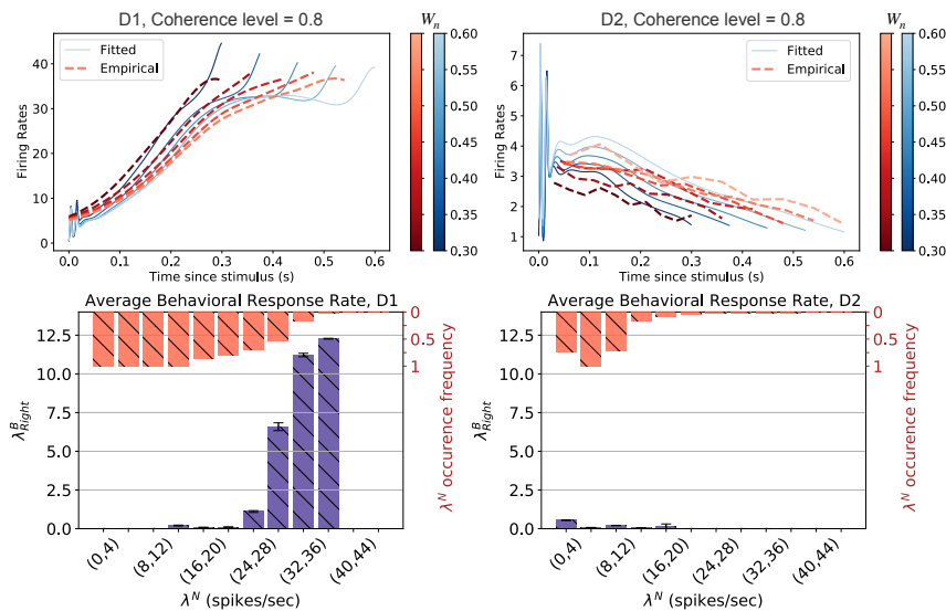
Figure 3: Synthetic Data (Upper panels). The activity rate of neural population in the two integrator regions of the synthetic dataset. The dashed lines show the empirically derived firing rates compared to the solid lines which are estimated using the proposed model. Each line plot corresponds to the average activity rate of trials with W_n in a specific interval illustrated by the colorbar (see section F in Supplementary Materials ). (Lower panels). Illustrating the average response rate for each interval of neural activity rates. The plots correspond to the trials with highest coherence level. The plots show the average between trials with a RIGHT reaction. Error bars show the standard error. Purple bars show the average behavioural response rates. Orange bars indicate the proportion of trials with the occurrence of each neural response interval.
