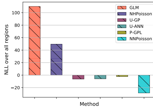
Figure 5: Total NLL of the estimated neural intensity function on Steinmetz test set. Illustrating the sum of NLL values evaluated over all the 37 test regions in the Steinmetz dataset using different baselines compared to the performance of the proposed method.
