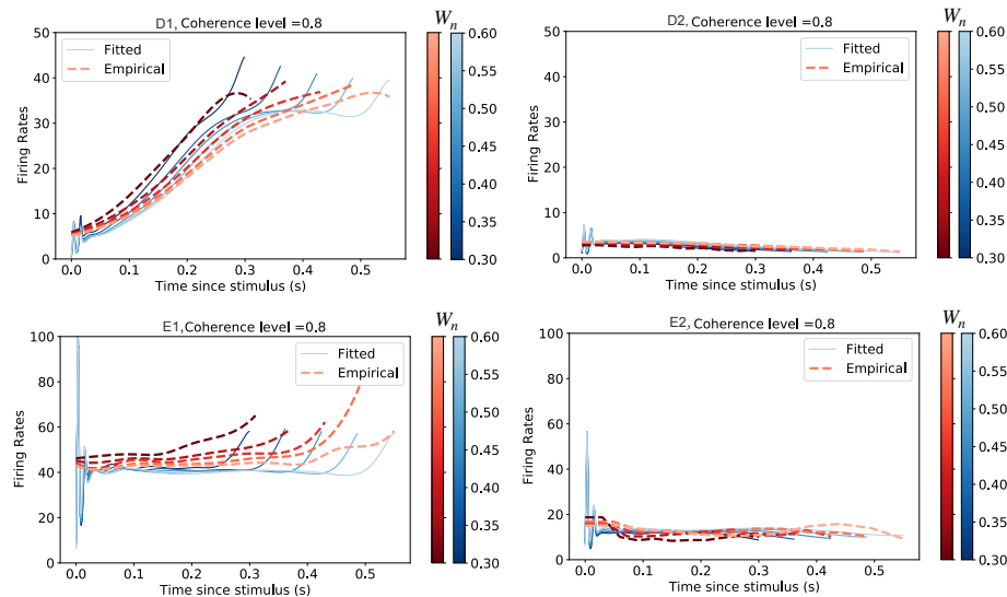
Figure 8: Synthetic Dataset. The red dashed lines are the empirically derived firing rates compared to the blue solid lines which are estimated using the proposed model. The plots correspond to the trials with high contrast on RIGHT. As expected from the dataset architecture, for trials when the RIGHT choice is made, the activity in D1 represents an increasing trend until the response is made. This is in contrast with region D2 for these trials where there is little to no activity detected in this region. Neurons in both sensory regions, E1 and E2 show constant activity throughout each trial with higher activity detected by E1 neurons which prefer rightward motion.
