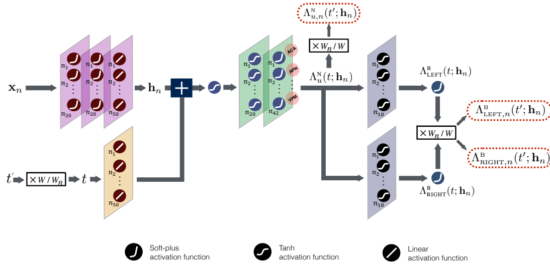
Figure 7: Model Architecture. Schematic representing the details of the implemented neural network to be trained on the Steinmetz dataset. The neural and behavioural outputs of this network are multiplied by a factor of W_n/W for the selected linear transformation function, z , to obtain the final model readouts.
