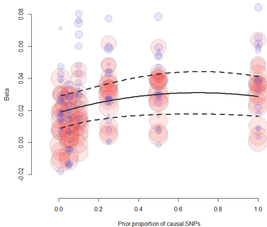
Supplementary Figure 1: Bubble plot of the relationship between the polygenicity prior and the effects size in the polygenic risk score analyses. Not the increase in effect size with the increase in polygenicity prior. The solid line indicates the best fit obtained from the meta-regression model (model 3) where the dashed lines reflect the upper and lower confidence bounds.
