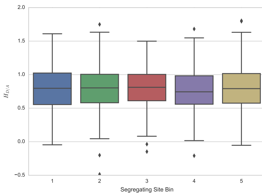
Figure S9: H_{D/A} plotted against quintiles of segregating sites in 1,000 simulations.
