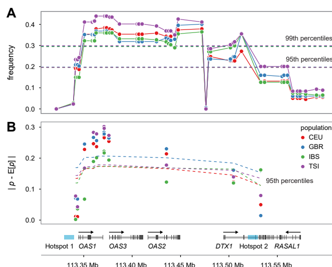
Figure 2: OAS-introgressed haplotypes are found at higher frequencies in European populations than expected under neutrality. (A) Comparison of frequency (y-axis) of NLS in the OAS locus in the CEU, GBR, IBS, and TSI European population samples with respect to neutral expectations (dashed lines) based on coalescent simulations. (B) Absolute difference between observed and expected allele frequency in the same four present-day European samples (y-axis) based on ancient DNA data. Dashed lines represent the 95 th percentile of the expected distribution based on similar deviations calculated on a dataset of approximately one million SNPs scattered around the genome and with comparable present-day frequencies to those found for NLS in the OAS region.
