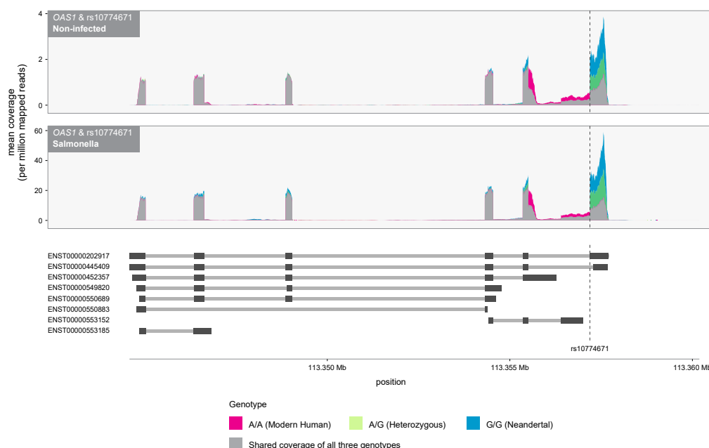
Figure S6: The splicing variant rs10774671 is a strong asQTL for OAS1 . Plotted is the normalized average coverage at which each base was sequenced along the genomic regions encoding the gene OAS1 . Individuals were stratified according to their genotype at rs10774671. Below the figure are gene models from the Ensembl database. Individuals carrying the G allele at rs10774671 (i.e. the Neandertal allele) primarily express the transcript ENST00000202917 (referred to as p46 in the text) whereas individuals carrying the A derived allele lose the splice site, which leads to the usage of a distinct isoform.
