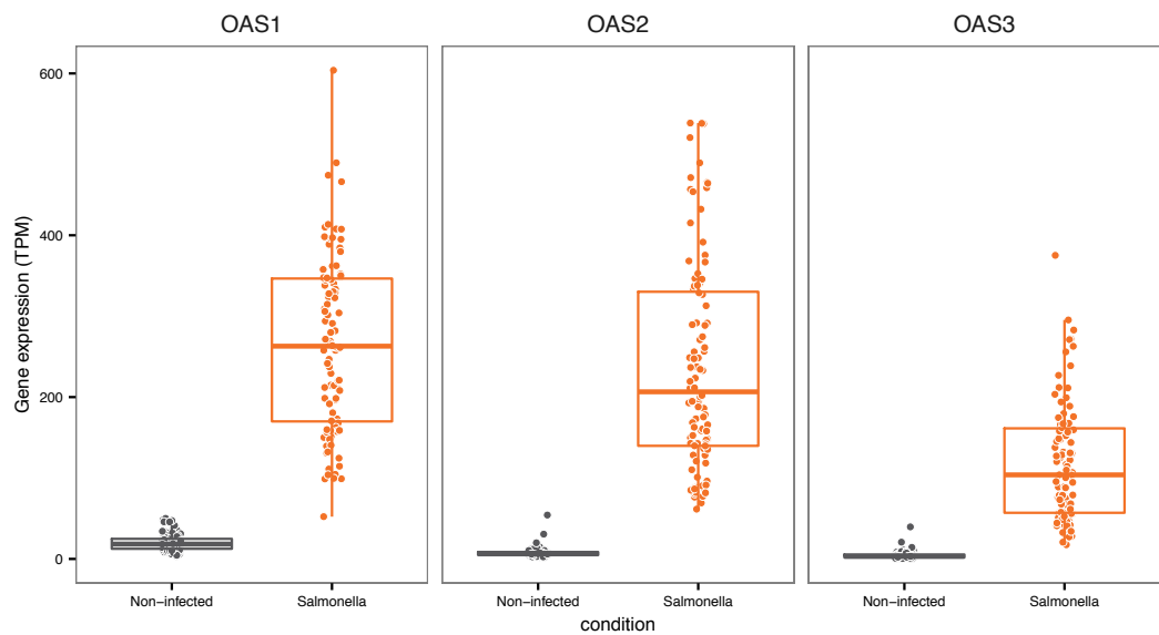
Figure S5: Expression levels of OAS genes in primary macrophages (European) before and after infection with Salmonella.
