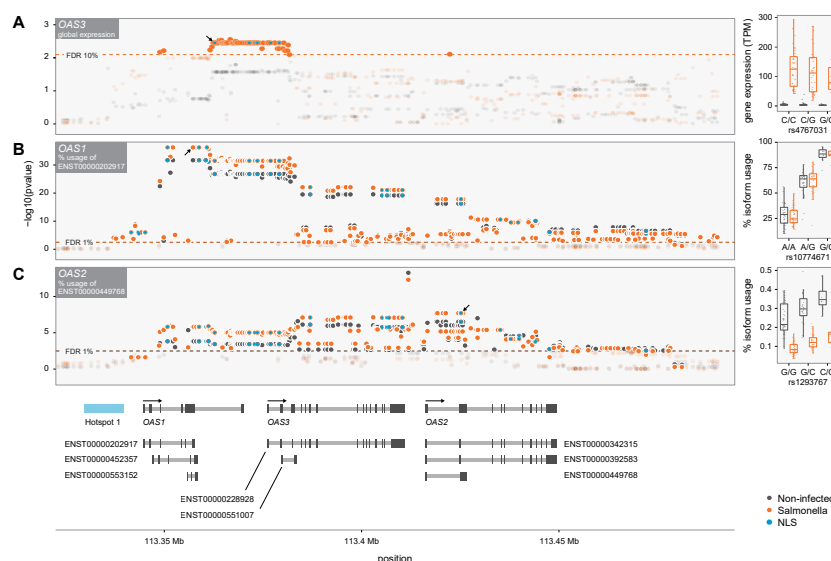
Figure 4: Pervasive impact of the Neandertal haplotype on the regulation of OAS genes in primary macrophages. (A) -\log_{10} P s (y-axis) for the association between genotypes for SNPs with a MAF > 10% in the OAS region and expression levels of OAS3 in non-infected (black) and Salmonella -infected macrophages (orange). The dashed line shows the P cutoff corresponding to an FDR of 10%. The right panel shows a boxplot for the association between genotypes at the NLS rs4767031 (x-axis) and the expression levels of OAS3 in TPM (Transcripts Per Kilobase Million) (y-axis). The lower expression level of OAS3 in individuals harboring the Neandertal haplotype were confirmed by real-time PCR (Figure S11) (B) -\log_{10} P s (y-axis) for the association between genotypes in the OAS regions and the percentage usage of isoform ENST00000202917 (i.e., p46 in the text) in non-infected (black) and Salmonella -infected macrophages (orange). The dashed line shows the P cutoff corresponding to an FDR of 1%. The right panel shows a boxplot for the association between genotypes at the splicing variant rs10774671 (x-axis) and the percentage usage of isoform p46 (y-axis). (C) Similar
