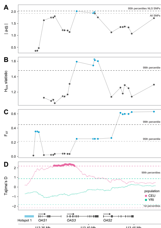
Figure 3: OAS-introgressed haplotypes show multiple signatures of positive selection. (A) Normalized absolute iHS scores (y-axis) across SNPs in the CEU sample. Dashed lines represent the 95 th percentile of iHS calculated genome-wide across all SNPs (grey) and all NLS SNPs (black). (B) The H_{D/A} statistic in CEU (y-axis). Dashed line indicates the 99 th percentile of H_{D/A} calculated across 1,000 simulations. (C) F_{ST} calculated between CEU and all East Asian populations from the 1000 Genomes projects (y-axis). Dashed lines indicate the 95 th (grey) and 99 th (black) genome-wide percentiles of F_{ST} . Similar results are obtained when comparing any other European population against East Asians (Table S5). (D) Tajima's D (y-axis) calculated for CEU and YRI samples. Dashed lines indicate the 1 st and 99 th genome-wide percentiles of Tajima's D.
