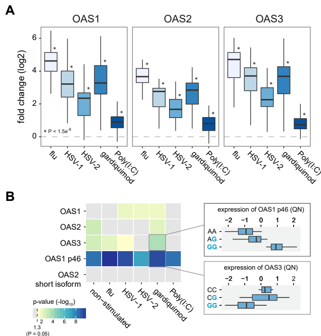
Figure 5: The Neandertal haplotype in the OAS regions has a different impact on the regulation of OAS genes depending on the viral agents PBMCs are exposed to. (A) Log 2 fold induction (y-axis) of OAS1 , OAS2 and OAS3 in response to different viral agents or viral-associated immune stimuli, relative to non-infected PBMCs (B) -\log_{10} P for the association between genotype status for the Neandertal haplotype and overall expression levels of OAS genes and the expression of specific isoforms of OAS1 and OAS2 (those identified in Figure 3 as associated with NLS). Boxplots show the association between genotype status (blue referring to Neanderthal alleles) and expression levels of the p46 isoform of OAS1 and OAS3 in Gardiquimod-stimulated PBMCs.
