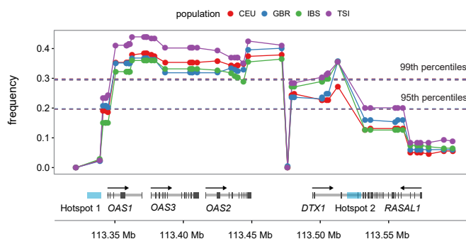
Figure S3: OAS-introgressed haplotypes are found at higher frequencies in European populations than expected under neutrality when using a two-pulse introgression model. (A) Comparison of frequency (y-axis) of NLS in the OAS locus in the CEU, GBR, IBS, and TSI European population samples with respect to neutral expectations (dashed lines) based on coalescent simulations considering two-pulse introgression in both Europeans and Asians, or a second pulse of introgression only in Europeans. Dashed lines overlap almost completely, reflecting little variation between a two-pulse introgression in both European and Asians, or a second pulse only in Europeans.
