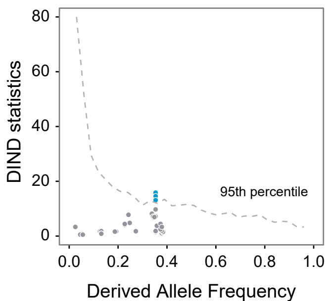
Figure S4: The DIND statistic indicates reduced diversity surrounding NLS. DIND (y-axis) is plotted for SNPs in OAS locus by derived (Neandertal) allele frequency. Dashed line indicates genome-wide 95 th percentile by frequency.
