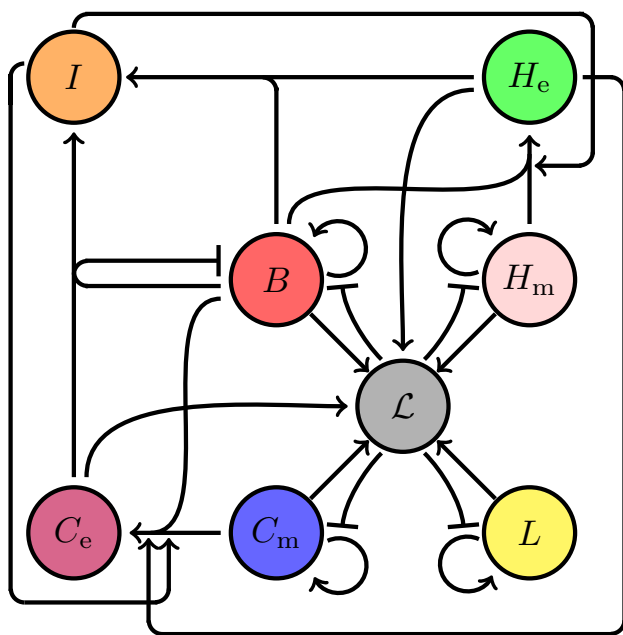
Figure 2: Schematic representation of key interactions. CAR-modified effector CTLs ( C_e ), upon encountering B cells ( B ), secrete inflammatory cytokines ( I ) and cause lysis in B cells. Inflammation increases the rate at which CAR-modified memory CTLs ( C_m ) and memory Helper T cells ( H_m ) become effector cells. CAR-modified effector Helper T cells ( H_e ) further increase the rate at which memory CTLs become effectors, and secrete inflammatory cytokines when they encounter B cells. The total number of lymphocytes ( \mathcal{L} ) increases when any one of the lymphocyte populations increases. Memory cells ( H_m , C_m ) and other endogenous lymphocytes ( L ) undergo homeostatic division in response to lymphopenia, and B cells proliferate whenever \mathcal{L} is below the carrying capacity.
