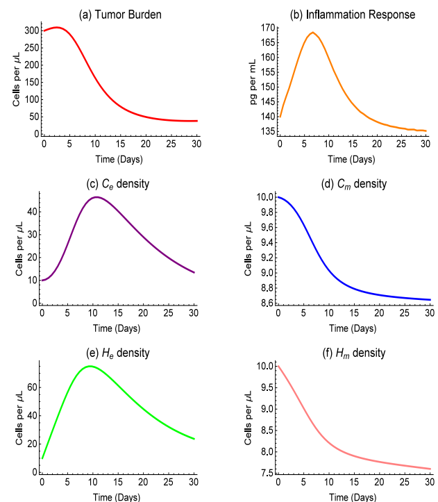
Figure 3: Simulated patient response: A simulated standard patient is administered CAR T cells on day 0 and monitored over 30 days. The tumour burden is depicted in (a), the inflammatory response in (b), and respective T cell populations are depicted in (c)-(e) inclusive. Simulation details are outlined in the text.
