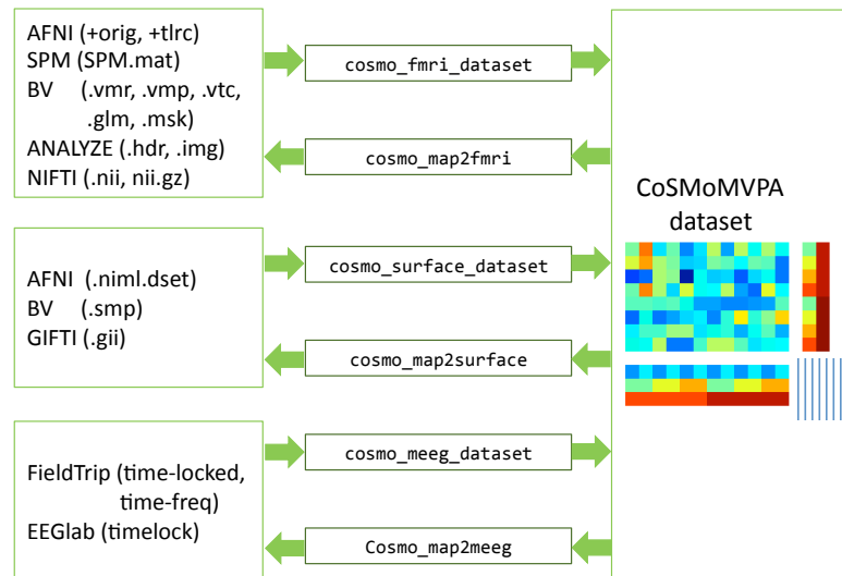
Fig. 10: Dataset input/output support
