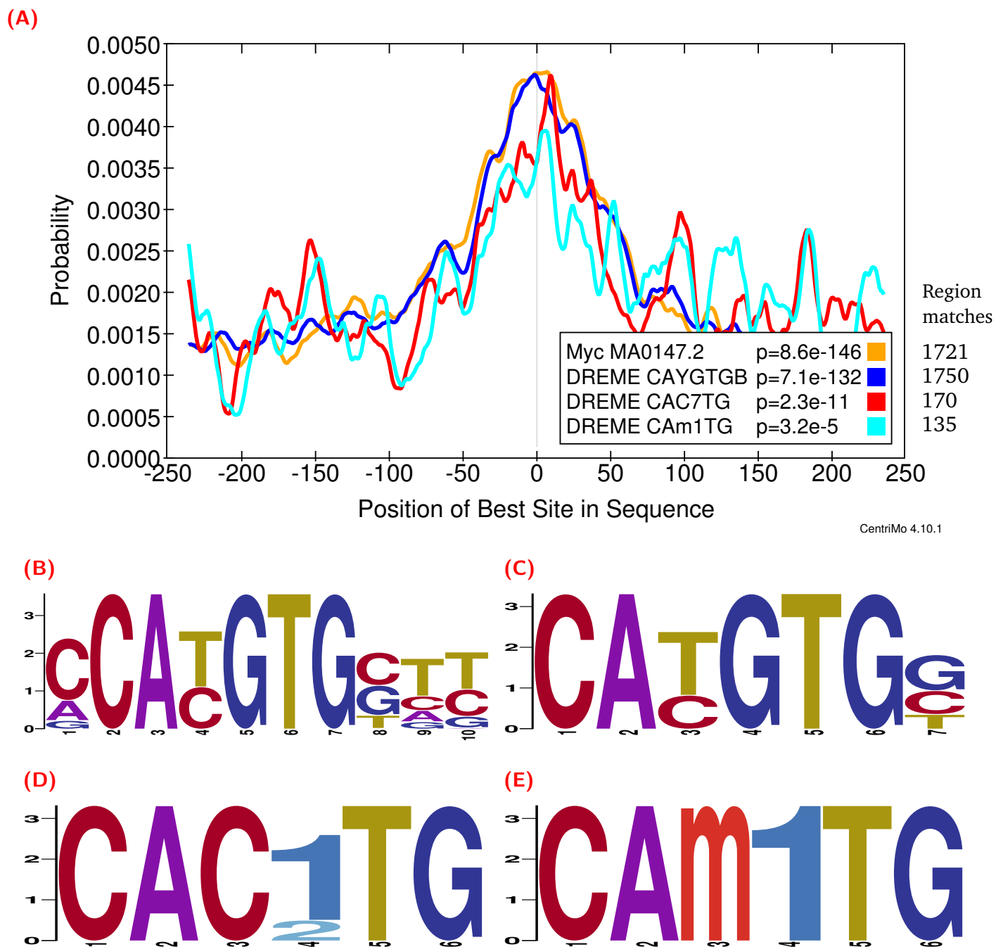
Figure S4. c-Myc (ENCF001YJE; 6297 ChIP-seq peaks) CentriMo analysis upon de novo and JASPAR motifs (see Methods ) using female replicate 2 of the (ox)WGBS data 51 at a 0.7 modification threshold. (A) the CentriMo result with the c-Myc JASPAR motif in orange (logo in (B)), a top E-box unmodified motif in blue (logo in (C)), and DREME (hydroxy)methylated motifs in red and cyan (logos in (D) and (E), respectively). We depict the JASPAR sequence logo using MEME's relative entropy calculation and colouring for consistency.
