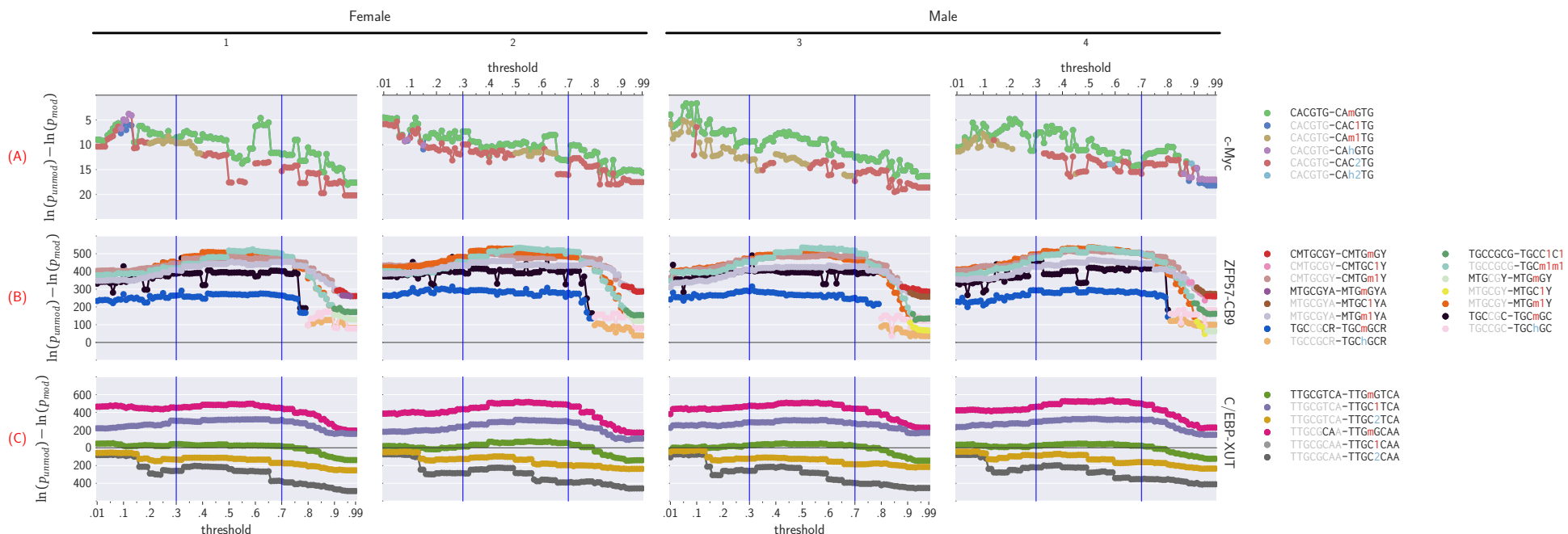
Figure 5. Relationship between unmodified versus modified motif statistical significance of central enrichment (from CentriMo 66 ) and modified base calling thresholds across different (ox)WGBS specimens. 51 Each unmodified motif, at each threshold, is compared to its top three most significant modifications for c-Myc and C/EBP \beta , but top one most significant modification for ZFP57. Since at most the top three motif pairs are selected per threshold value, specific thresholds can result in new motif pairs, while previously enriched pairs may no longer be present at a given threshold. Each column pertains to a particular (ox)WGBS replicate. Each row of plots pertains to a single ChIP-seq replicate for a particular transcription factor target, one each of: c-Myc (Krepelova et al. 75 ), ZFP57 (CB9; Strogantsev et al. 38 ), and C/EBP \beta (ENCF001XUT). Negative values correspond to a preference for the unmodified motif, while positive values correspond to a preference for the modified motif.
