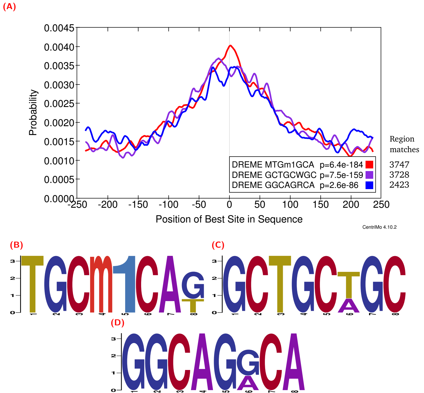
Figure S5. Strogantsev et al. 38 CB9 ZFP57 (mm9 aligned; 72 592 ChIP-seq peaks) CentriMo analysis upon de novo and JASPAR motifs (see Methods ) using female replicate 2 of the (ox)WGBS data 51 at a 0.7 modification threshold. (A) the CentriMo result with an expected ZFP57 modified motif in red (logo in (B), reverse complement shown) and top unmodified motifs in purple (logo in (C)) and blue (logo in (D)).
