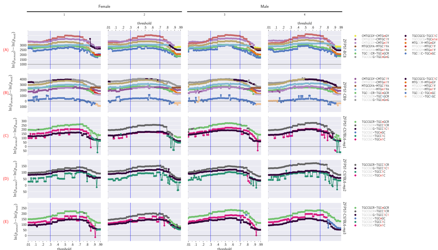
Figure S2. Relationship between unmodified versus modified motif statistical significance of central enrichment (from CentriMo 66 ) and modified base calling thresholds across different (ox)WGBS specimens. 51 Each unmodified motif, at each threshold, is compared to its top most significant modification. Since only the top motif pair is selected per threshold value, specific thresholds can result in new motif pairs, while previously enriched pairs may no longer be present at a given threshold. Each column pertains to a particular (ox)WGBS replicate. Each row of plots pertains to a particular ZFP57 ChIP-seq dataset: Strogantsev et al. 38 BC8 cells, Strogantsev et al. 38 CB9 cells, Shi et al. 80 (3 replicates). All ZFP57 peaks were called using the default MACS 76 peak calling threshold, q = 0.05 . Negative values correspond to a preference for the unmodified motif, while positive values correspond to a preference for the modified motif.
