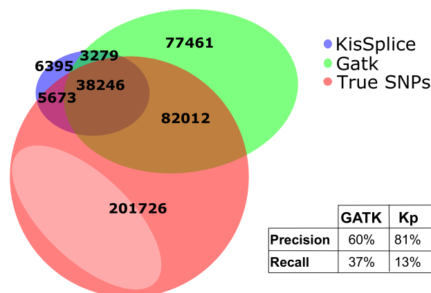
Figure 5: Precision and recall of KISSPLICE and GATK. Half of the SNPs found by no method are covered by less than 10 reads (in light red).
