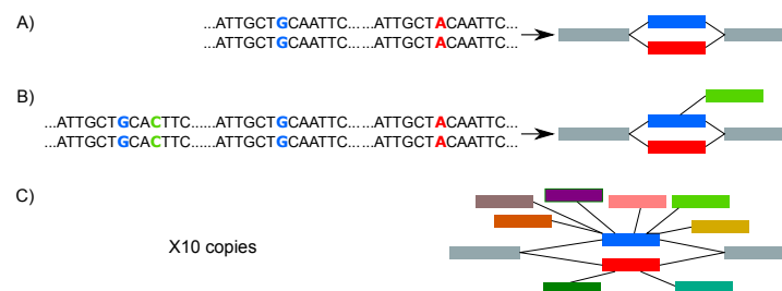
Figure 4: Two inexact repeats give rise to a pattern in the DBG that resembles a SNP (A). Very often, repeats are present in more than 2 copies (B) and therefore generate branching bubbles. Bubbles with more than 5 branches (C) are filtered out.
