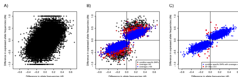
Figure 6: Difference of allele frequencies ( df ) Vs Difference of expressed allele frequencies ( dfe ) A) All SNPs B) Condition Specific SNPs C) Conditions Specific SNPs covered by at least 100 reads.
