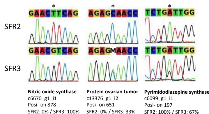
Figure 8: SNPs validated by Sanger sequencing. The first is fixed in both SFR2 and SFR3 lineages. The second and the third are polymorphic in SFR3
