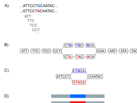
Figure 2: A) A SNP present in two alleles in the data. B) The de Bruijn Graph derived from the data. For the sake of simplicity of exposition, we draw here with k=3 . In practice, k=41 . C) A compressed de Bruijn Graph can be obtained by merging nodes with a single outgoing edge with nodes with a single incoming edge. This compression step is lossless. D) The two paths in the compressed de Bruijn Graph correspond to the two alleles of the SNP.
