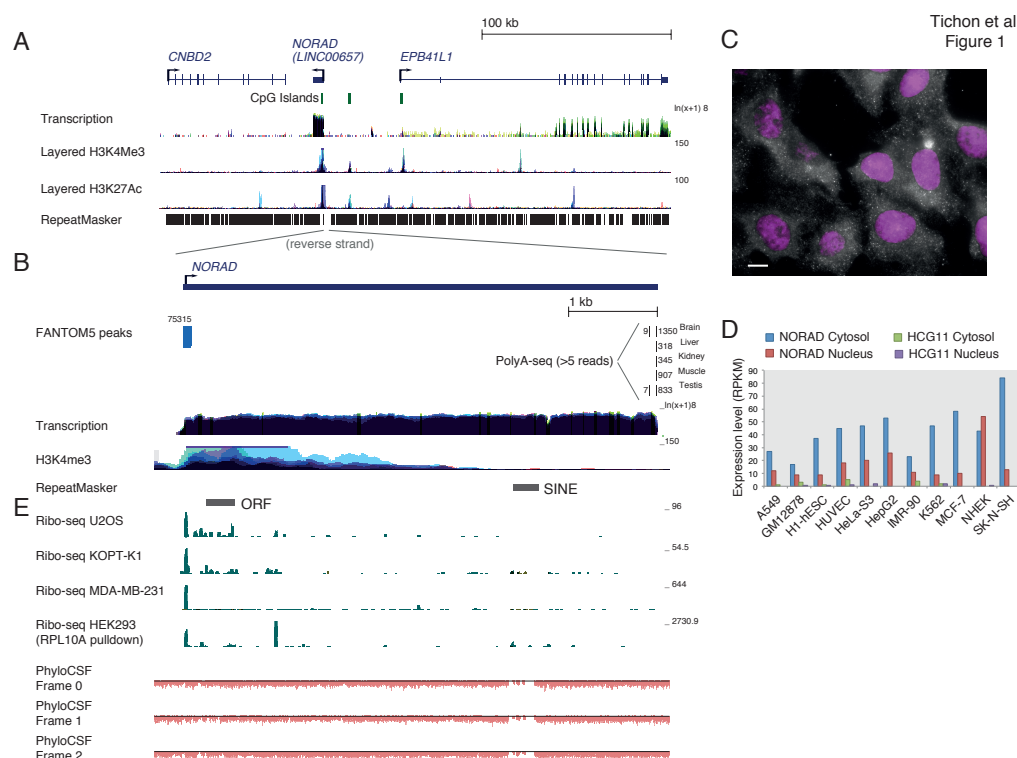
Figure1. Overview of the human NORAD locus. (A) Genomic neighborhood of NORAD. CpG island annotations and genomic data from the ENCODE project taken from the UCSC genome browser. (B) Support for the transcription unit of NORAD. Transcription start site information taken from the FANTOM5 project 43 . Polyadenylation sites taken from PolyA-seq dataset 44 . ENCODE datasets and repeat annotations from the UCSC browser. (C) Predominantly cytoplasmic localization of NORAD by smFISH. Scale bar 10µm. See Supplementary Fig. 2 for RNA-FISH following NORAD knockdown. (D) Estimated copy number of NORAD in 22 independent cells from two independent experiments. (E) Expression levels of NORAD and HCG11 in the ENCODE cell lines (taken from the EMBL-EBI Expression Atlas ( https://www.ebi.ac.uk/gxa/home )). (E) Support for the noncoding nature of NORAD. Ribosome protected fragments from various human cell lines (MDA-MB-231 22 , HEK-293 23 , U2OS 24 , KOPT-K1 25 ) mapped to the NORAD locus and PhyloCSF 45 scores. All PhyloCSF scores in the locus are negative.
