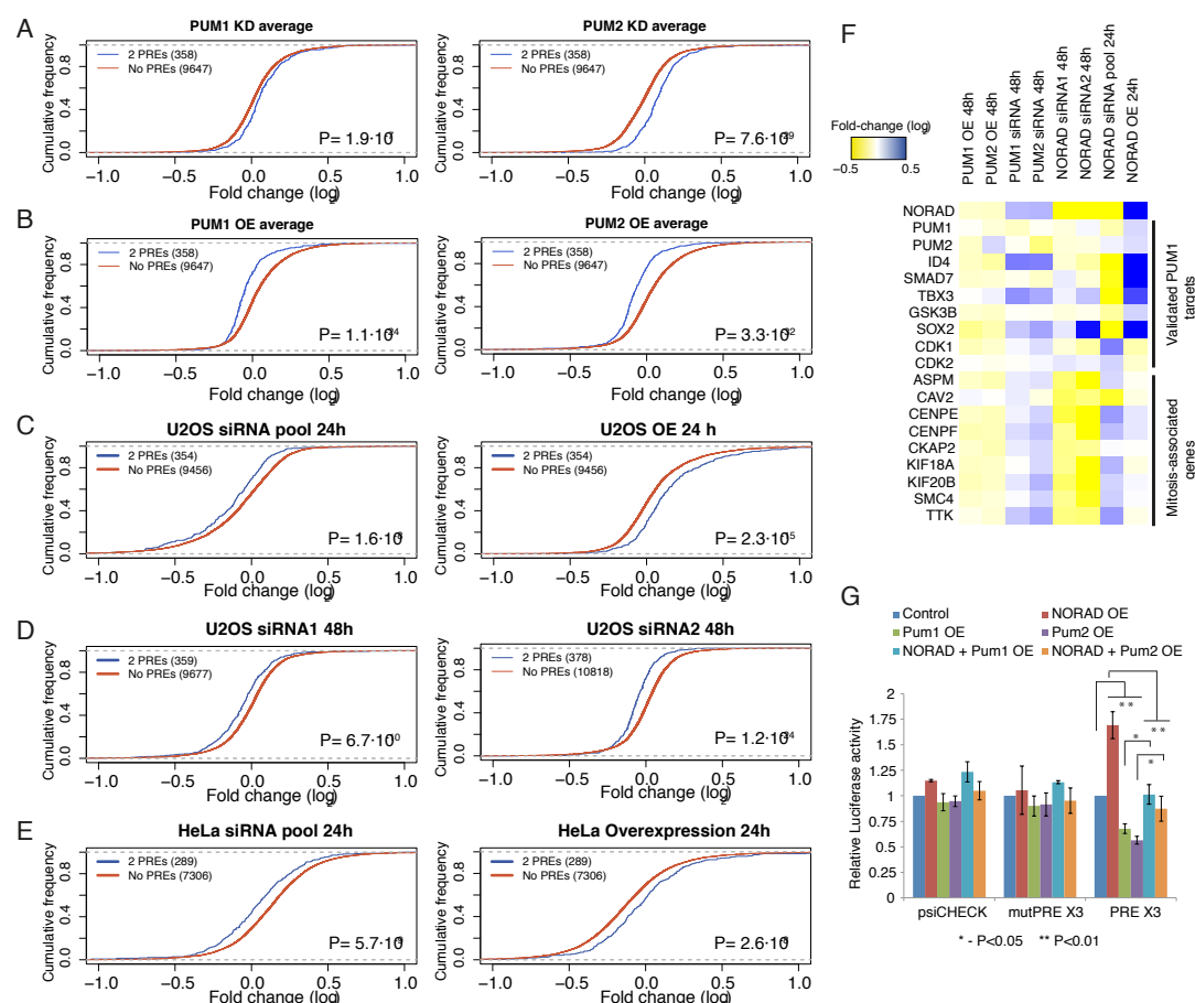
Figure 4. NORAD modulates expression of Pumilio targets. (A-E) Changes in expression of Pumilio targets compared to controls, following the indicated treatment. “2 PREs” are genes that contain at least two canonical PREs over what is expected by chance in their 3' UTRs, “Controls” are those genes that do not contain more sites in their 3' UTRs than expected by chance. (F) Changes in expression of NORAD, PUM1/2, validated targets of PUM1 31 and genes with annotated roles in the M phase of the cell cycle and/or the mitotic spindle following the indicated perturbations. (G) Changes in luciferase activity measured from the indicated vectors following over-expression of the indicated genes and combinations.
