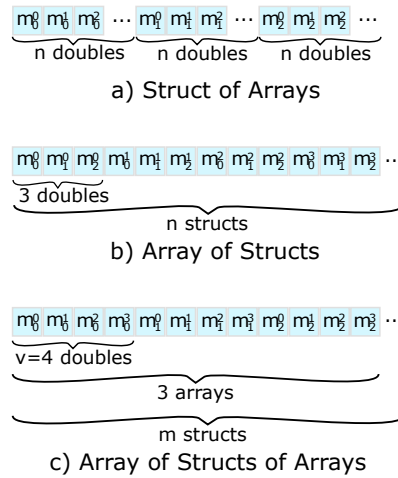
Fig. 3. Alternative data layouts for storing anti-diagonals
