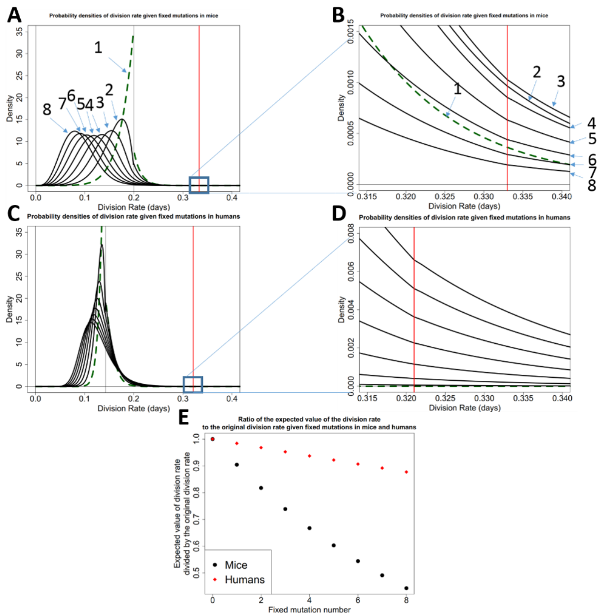
Figure 2. The accumulation of probability densities describing stem cell division rate. A: Exponentially distributed fitness effects on division rate using the parameters in Table 1 for the mouse. The first density is a green dashed line. Each probability density represents the division rate of a fixed lineage after n fixed mutations, with n indicated by an arrow. B: Zooming in on the tumorigenesis threshold, we see that the area of the division rate density that is over the tumorigenesis threshold increases at first and then decreases with subsequent mutation. There is a change in slope of the densities at the tumorigenesis threshold because subsequent densities are calculated from the previous density which has had the area to the right of the tumorigenesis threshold removed and the area to the left renormalized to 1. C,D are the same as A and B , respectively, but are for the human scenario. The larger population size decreases the strength of drift. Order of mutations in C proceeds as in A , and proceeds from 1 through 8 from bottom to top in D . E: The expected values of the probability densities in A and B divided by their original values over subsequent fixed mutations
