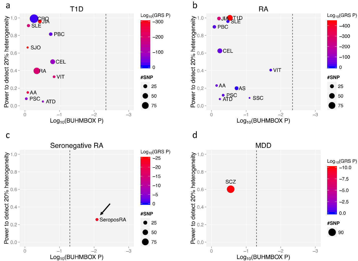
Figure 6. BUHMBBOX results. Dashed vertical lines denote the Bonferroni-adjusted significance threshold.
