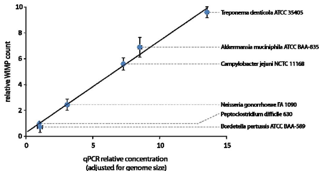
Figure 1. Comparison of WIMP read counts with quantitative PCR measurements
