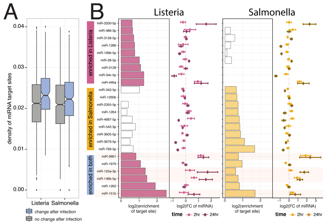
Figure 6. Tandem 3' UTR shortening allows evasion of regulation by miRNAs.
