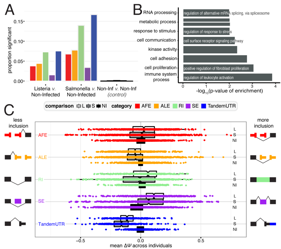
Figure 2. RNA processing changes in response to bacterial infection. (A) Proportion of events for RNA processing category that are significantly changing after infection with Listeria (left), Salmonella (middle), or variation between non-infected samples as a control (right). Numbers indicate the number of significant changes per category. (B) Significantly Gene Ontology categories for genes with any significant RNA processing change (FDR \leq 10\% ). (C) Distribution of \Delta\Psi values for each RNA processing category. Negative values represent less inclusion, while positive values represent more inclusion, as defined by the schematic exon representations.
