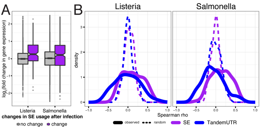
Figure 5. Relationship between RNA processing changes and gene expression changes. (A) Distribution of fold changes in gene expression ( y -axis, log 2 scale) for genes with significant skipped exon changes after infection ( purple ) and genes with no change after infection ( gray ). (B) Distribution of Spearman correlations between \Delta\Psi and fold change in gene expression across 60 individuals per gene ( solid line ), for genes with only one annotated alternative event and significantly changed SE usage ( purple ; n_L = 46 genes and n_S = 97 genes) or tandem UTR usage ( blue ; n_L = 36 genes and n_S = 86 genes). Dotted lines show distribution of the correlation coefficients after permuting \Delta\Psi values.
