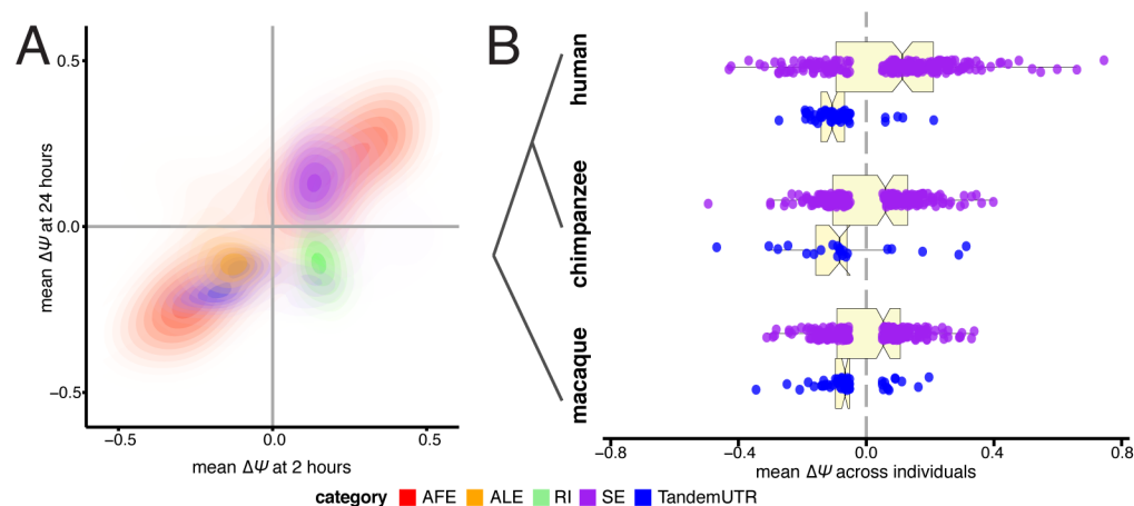
Figure 4. Directed shifts in RNA processing persist across time, stimulus conditions, and closely related species. (A) Correlations between \Delta\Psi values after 2 hours of infection ( x-axis ) and \Delta\Psi values after 24 hours of infection ( y-axis ), presented as density plots per RNA processing category in contrasting colors. Plotted are events that are significant after 2 hours of either Listeria or Salmonella infection. (B) Distributions of \Delta\Psi values for skipped exons ( purple ) and TandemUTRs ( blue ) following infection of whole blood cells with lipopolysaccharide, assessed in human ( top ), chimpanzee ( middle ) and rhesus macaque ( bottom ) individuals ( N=6 per species). We observe prominent global shifts in isoform distributions in human and macaque ( SE_{human} P=0.003 , TandemUTR_{human} P=2.4\times 10^{-13} ; SE_{macaque} P=0.05 , TandemUTR_{macaque} P=8.8\times 10^{-6} ) with a more modest trend observed in chimpanzee, potentially due to poor transcript annotations in the chimpanzee genome ( SE_{chimpanzee} P=0.26 , TandemUTR_{chimpanzee} P=0.002 ). All p-values were calculated using a Student's t-test testing deviation from a mean of zero.
