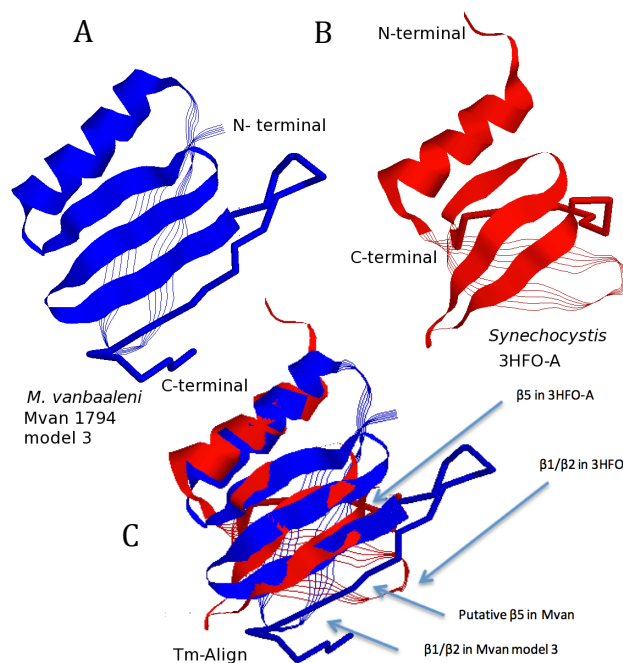
Figure 4. Comparison of the tertiary structures for (A) Mycobacterium vanbaalei Mvan_1794 DUF3107 (Mvan_model3.pdb) (B) Synechocystis sp. PCC 6803 hfq (C) Aligned structures (Tm-align 27 ). Aligned structures ( \alpha 1 and \beta 2ii/\beta 3/\beta 4 ) are displayed as ribbon. The \beta 1/\beta 2i sheet as strands and \beta 5 in 3HFO-A, and the putative \beta 5 and extended C-terminal in Mvan_1794, as backbone.
