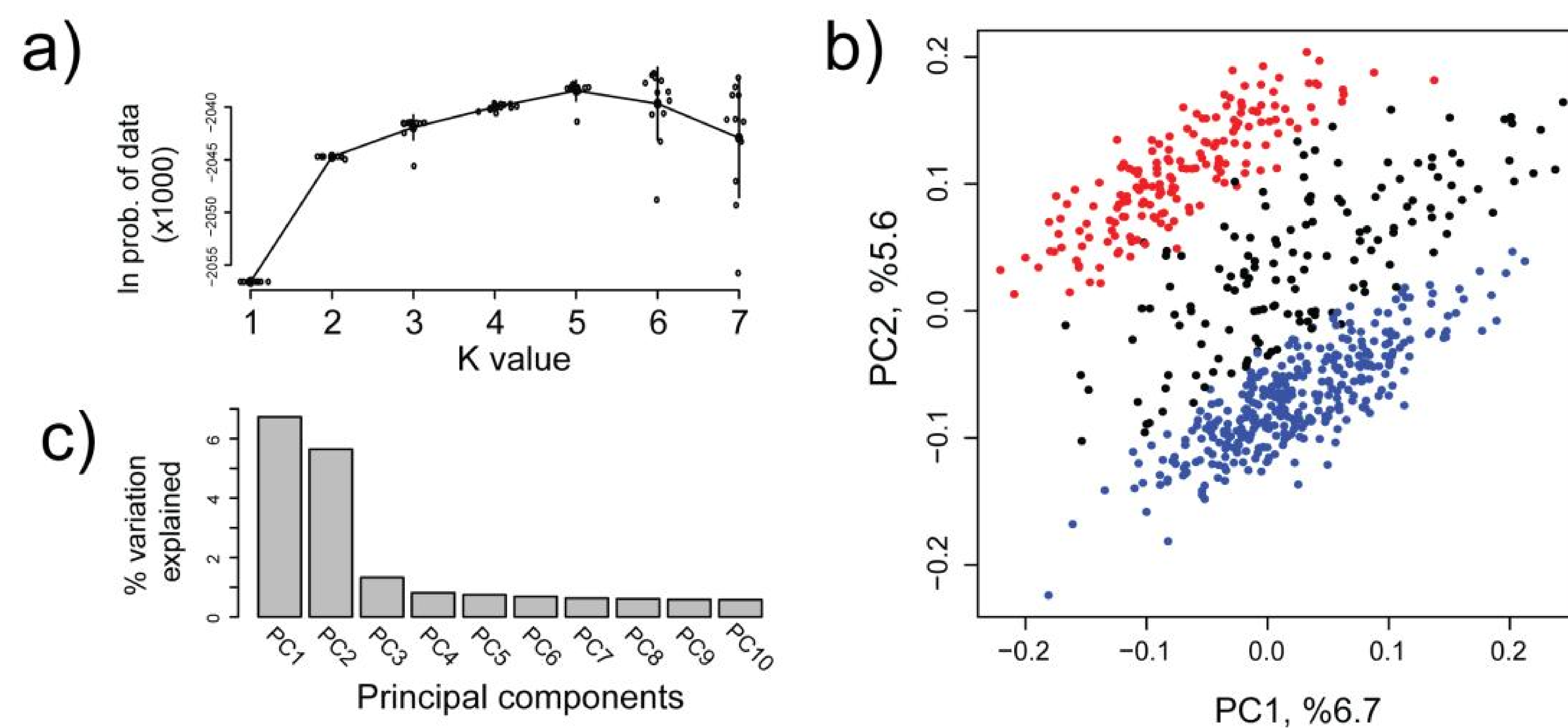
Figure 2: STRUCTURE and principal component analyses of Atlantic salmon sampled from the Teno River mainstem. a) The estimated \ln probability of data given the K value. Error bars are standard deviations of 12 replicate runs. The results for each of the 12 replicate runs are given with smaller circles; b) Plot of the first two major PC axes, where colors show sub-populations inferred by the STRUCTURE analysis at the optimum K value of two. Blue, red and, black colors show Sub-population 1, Sub-population 2, and admixed individuals, respectively. (c) Percent variation explained by the first 10 PC axes.
