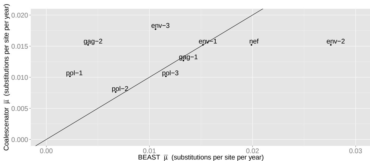
(A) Comparison of BEAST's and Coalescentor's mutation rate \bar{\mu} estimates
