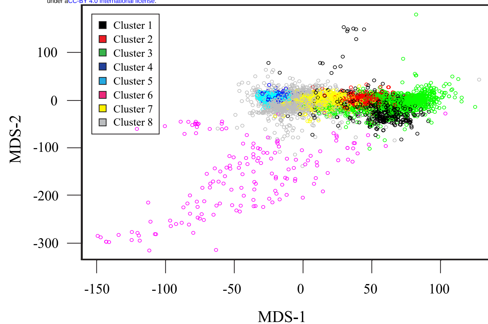
Figure 4: Hierarchical clustering results using L1 distance and Ward's method shown as (A) a dendrogram and (B-C) in multi-dimensional scaling plots. (A) The horizontal dotted red line shows the cut-off at a cluster dissimilarity index of about 10000, which results in 8 clusters. The clusters are number 1 to 8 from left to right, with 4 and 5 containing primarily non-SVs, 8 containing a mixture of SVs and non-SVs, and 1, 2, 3, 6, and 7 containing different types of deletions (see Table 4). (B-C) Multidimensional scaling plots for visualizing the 8 clusters. We use a 3 dimensional representation of the data space which associates 3 MDS coordinates to each site, one for each dimension. (B) Plot of MDS-2 against MDS-1, which clearly separates Cluster 6 (mainly SVs with inaccurate breakpoints). (C) Plot of MDS-3 against MDS-1, in which the different types of SVs are generally well-separated from each other and from non-SVs.
