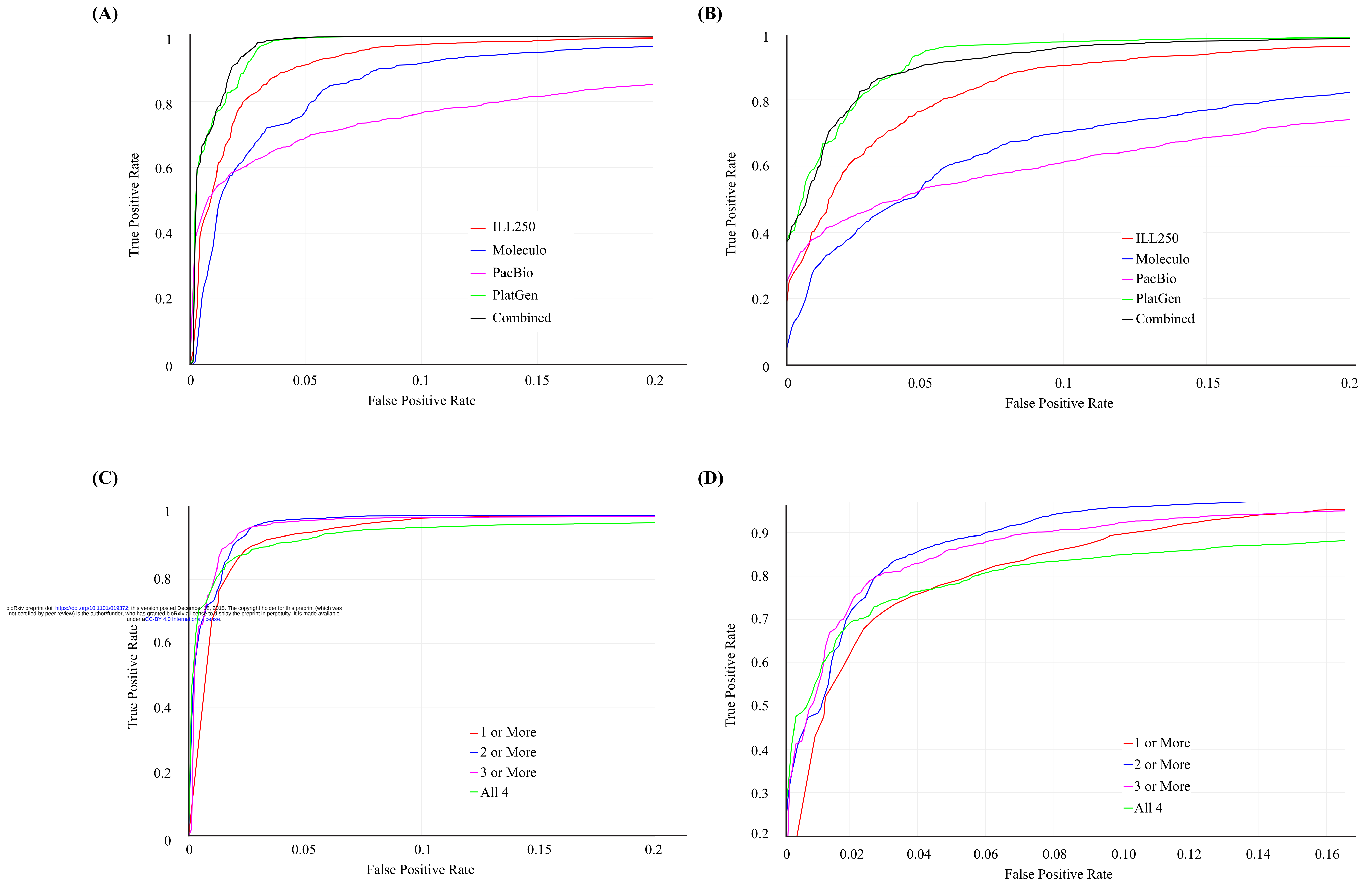
Figure 5: ROC curves for One-class classification using the L1 Distance, treating the 4000 Random regions as negatives and the Personalis or 1000 Genomes calls as positives. (A) ROC curves for one-class models for each dataset separately and for all combined for the Personalis validated deletion calls. (B) ROC curves for one-class models for each dataset separately and for all combined for the 1000 Genomes validated deletion calls. (C) ROC curves for one-class model requiring 1 or more, 2 or more, 3 or more, or all 4 technologies to have high classification scores for the Personalis validated deletion calls. (D) ROC curves for one-class model requiring 1 or more, 2 or more, 3 or more, or all 4 technologies to have high classification scores for the 1000 Genomes validated deletion calls. The 3 or more classification method is used to produce the final high-confidence SVs in this work. The horizontal axis shows the false positive rate (from the random set of regions matching the size distribution of the Personalis deletions) and the vertical axis shows the corresponding true positive rate (assuming all the validated/assembled calls are true). See original data at https://plot.ly/345/~parikhhm/ , https://plot.ly/353/~parikhhm/ , https://plot.ly/361/~parikhhm/ , and https://plot.ly/369/~parikhhm/ .
