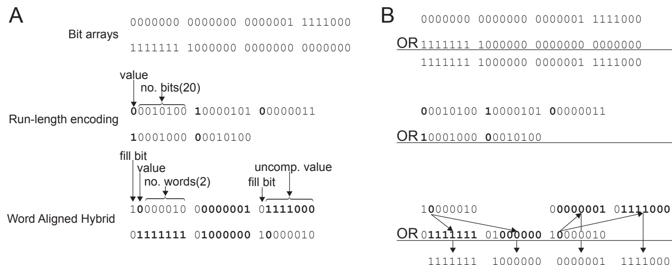
Figure S2. A comparison of binary encodings and associated bit-wise logical operations. (A) Two bit arrays are given in three different binary encodings: the uncompressed bit array on top, followed by the run-length encoding (RLE) and word-aligned hybrid encoding (WAH). RLE maps each set of consecutive bits to a new value that uses one bit for the run value, and the remaining bits for the number of bits in the run. WAH maps bits to one of two types of values: those that include runs and those that encode the raw binary. The first bit in a WAH value indicates if the value encodes a run (the fill bit). If that bit is set then the second bit gives the run value and the remaining bits give the run length in number of words (i.e., not number of bits as in RLE). If the fill bit is not set then the remaining bits are the uncompressed binary values. (B) The logical OR for the three encodings is given. For the uncompressed binary, the OR follows bit for bit across both values. For RLE, the logical OR is undefined (without inflation) because the two encoded values have different lengths. For WAH, the values are aligned based on their run length, then the logical OR is performed (in this case) between the value bit and the associated uncompressed values.
