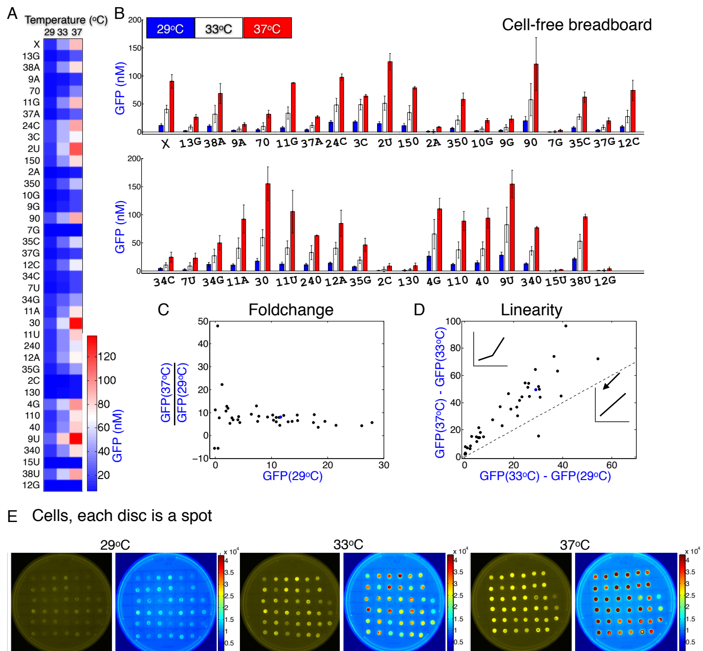
Figure 4: Experimental measurements of the thermometer library show a variety of responses. A. Rows represent activity levels of different thermometers. The activity levels are mean of three separate measurements. These values are normalised using a GFP calibration performed at 29°C. B. Replotting of data from A. Each set of three bars represents the activity levels of different thermometers. Blue, white, and red represent the temperatures 29°C, 33°C, and 37°C, respectively. The height of the bars corresponds the mean levels of three separate measurements with the standard deviation shown as the error bar. C & D. Each black dot represents a separate thermometer. A blue dot is used for the starting thermometer X. E. Thermometer activity in cell spots. Intensity represents green fluorescence. The identity of spots, read in a left-right, top-bottom manner, is the same as in A.
