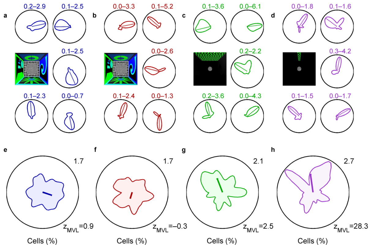
Figure 5: Bias of the neural ensemble by polarizing visual cues. a , Five example cells in RW_{rich} with significant directional tuning. The numbers indicate firing rate range. The dashed line corresponds to the preferred direction, i.e. the direction of maximum firing. The schematic in the middle left indicates the experimental condition. b–d , Same as in (a) but in VR_{rich} , VR_{polarized}^{wide} and VR_{polarized}^{narrow} conditions respectively. e , Distribution of preferred direction of neurons in RW_{rich} ( 341.71 \pm 4.66^\circ , n=278 , circular mean \pm circular s.e.m.). The number on the top right indicates the maximum value of the distribution. The thick blue line originating at the center of the polar plot represents both the direction ( 341.71^\circ ) and the magnitude (0.08) of the mean vector length of the preferred directions of the population (scaled by a factor of 5 for clarity). The mean vector length was not significantly different from chance ( z=0.95 ). f , Same as in (e) but for VR_{rich} . The distribution of preferred directions of neurons in VR_{rich} ( 253.27 \pm 5.97^\circ , n=174 , circular mean \pm circular s.e.m.) was not significantly different from that in RW_{rich} ( p=1 , circular Kuiper test). The mean vector length of the population (0.05) was not significantly different from chance ( z=-0.34 ). g , The ensemble of head-directionally modulated neurons in VR_{polarized}^{wide} ( 111.27 \pm 8.09^\circ , n=89 , circular mean \pm circular s.e.m.) were preferentially firing towards the visual cue ( p=0.04 , circular V test). Note the direction ( 111.27^\circ ) and the longer magnitude (0.12, z=2.50 which is significantly greater than chance) of the thick green line compared to (e, f). h , On the population level, neurons in VR_{polarized}^{narrow} ( 98.20 \pm 9.32^\circ , n=65 , circular mean \pm circular s.e.m.) were most biased towards the narrow cue ( p=0.04 , circular V test) as indicated by the magnitude (0.15, z=28.32 ) of the thick purple compared to all other conditions.
