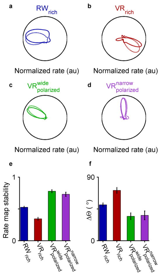
Figure 4: Stability of angular rate maps for head-directionally modulated neurons. a-d, Four directionally tuned cells with stable angular firing in the first half (solid colored lines) and second half (dashed colored lines) of the recording session. The peak rates are normalized for ease of comparison. e, Stability of the head-directional modulation (computed as the pairwise correlation between the angular rate maps in the first and second halves) in RW rich ( 0.53 \pm 0.02 , n=278 ) was significantly greater than VR rich ( 0.34 \pm 0.02 , n=174 , p=2.2 \times 10^{-9} , Wilcoxon rank-sum test here and throughout figure legend) but significantly smaller than VR wide_polarized ( 0.78 \pm 0.02 , n=89 , p=1.3 \times 10^{-16} ) and VR narrow_polarized ( 0.73 \pm 0.03 , n=65 , p=3.2 \times 10^{-9} ). Angular rate map stability was not significantly different between VR wide_polarized and VR narrow_polarized ( p=0.2 ). f, As an alternate measure of stability, we computed the absolute value of the circular distance between the preferred directions (defined as the direction of peak firing) in the two session halves. This method also resulted in a similar trend with VR wide_polarized ( 34.59 \pm 4.75^\circ ) and VR narrow_polarized ( 35.89 \pm 6.19^\circ ) showing identical levels of drift of the preferred directions ( p=0.5 ), both smaller than the amount of angular drift in RW rich ( 50.78 \pm 2.94^\circ , p=4.3 \times 10^{-5} and p=1.1 \times 10^{-4} respectively) and VR rich ( 71.16 \pm 4.23^\circ , p=1.4 \times 10^{-8} and p=4.7 \times 10^{-7} respectively).
