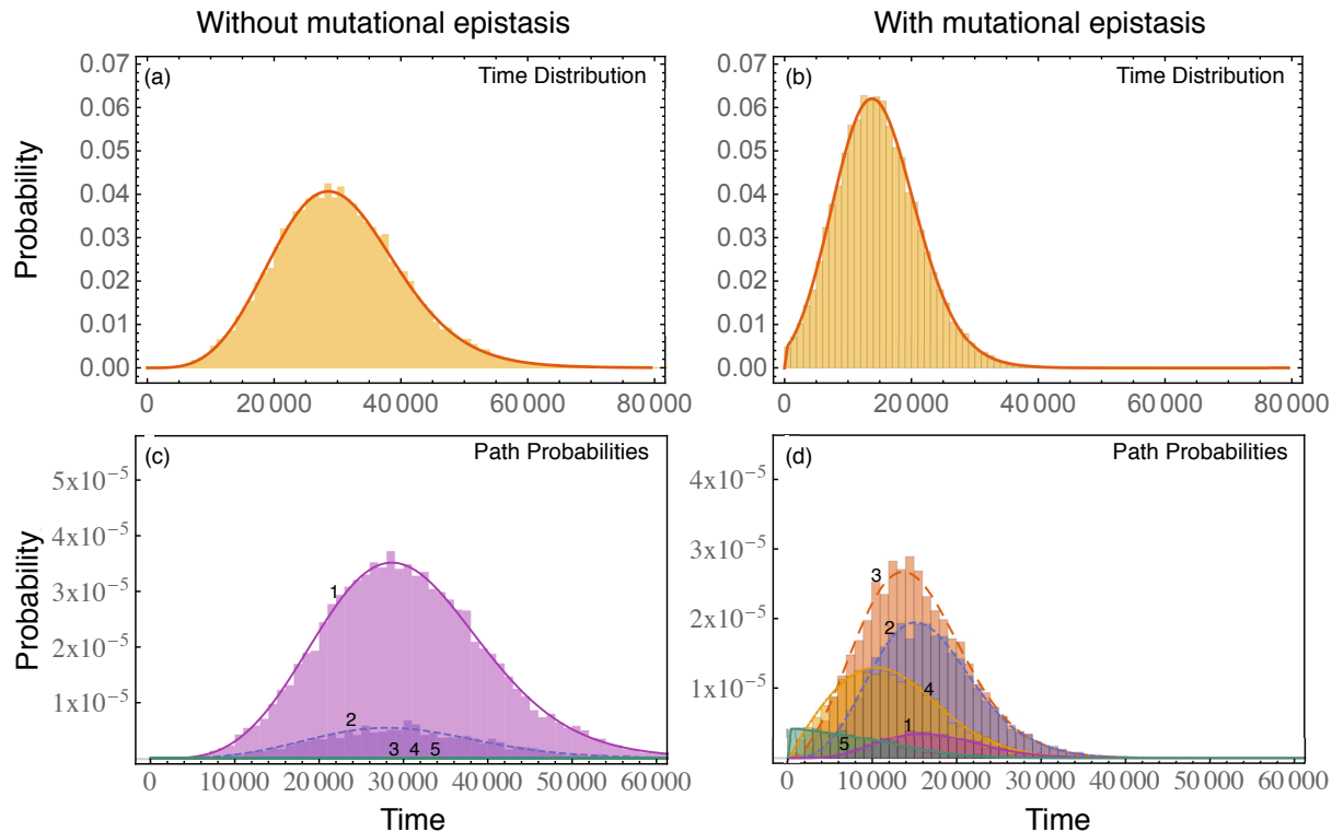
FIG. 5. Comparison between the path probability distributions of a minimal Burkitt Lymphoma model. Top: Time distributions for the model (a) without epistatic effects on mutation probabilities and (b) with mutational epistasis. The probability to obtain an A mutation is 100 times higher, if the B mutation is present in that individual. Bottom: In (c) the path probabilities for the model without epistatic effects on mutations are illustrated, whereas in (d) the mutation probability is again increased by 100 for an A mutation if the B mutation is present. Pathway 1 corresponds to the mutational pathway, where first all necessary extra mutations have to be acquired, and the B mutates last. Pathway 2 denotes the pathway, where 3 of 4 extra mutations have been obtained, then the B mutation happens, and at last the final extra mutation is acquired. Respectively for the other pathways (cf. Figure 4). The parameters are the same as in [28]: The birth probability for an individual with j passenger mutations and without the B mutation is b_{0,j} = 0.5(1 + 10^{-5})^j , and with the B mutation b_{1,j} = \frac{1.05}{2.2} \cdot 1.015^j . The mutation probability for the B mutation is \mu_D = 5 \cdot 10^{-6} , for an A mutation without the B mutation being present \mu_P = 2 \cdot 10^{-5} , and with the B mutation being present (only necessary for (b) and (d)) \mu_D^P = 2 \cdot 10^{-5} . The population size in the beginning is N = 500000 .
