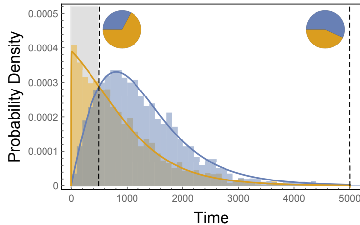
FIG. 3. Probability distribution for the different pathways. Orange represents the pathway via aB and blue the pathway via Ab . The bars are the results of simulations, the solid lines depict the computed results. In the pie charts the distribution of the pathways are illustrated up to 500 time steps (shaded area, left pie chart) and up to 5000 time steps (right pie chart). Stopping after a few lineages have reached the final mutant might lead to a false distribution: The other pathway might just need longer, but have a smaller extinction probability. The parameters are: Death probabilities: d_{ab} = 0.5, d_{aB} = 2/3, d_{Ab} = 0.49995, d_{AB} = 0.25 . Birth probabilities are 1 minus the corresponding death probability. Mutation probabilities are \mu_B = \mu_B^A = 2 \cdot 10^{-6}, \mu_A = 2 \cdot 10^{-5}, \mu_A^B = 0.005 . Initial Population size is N = 30000 .
