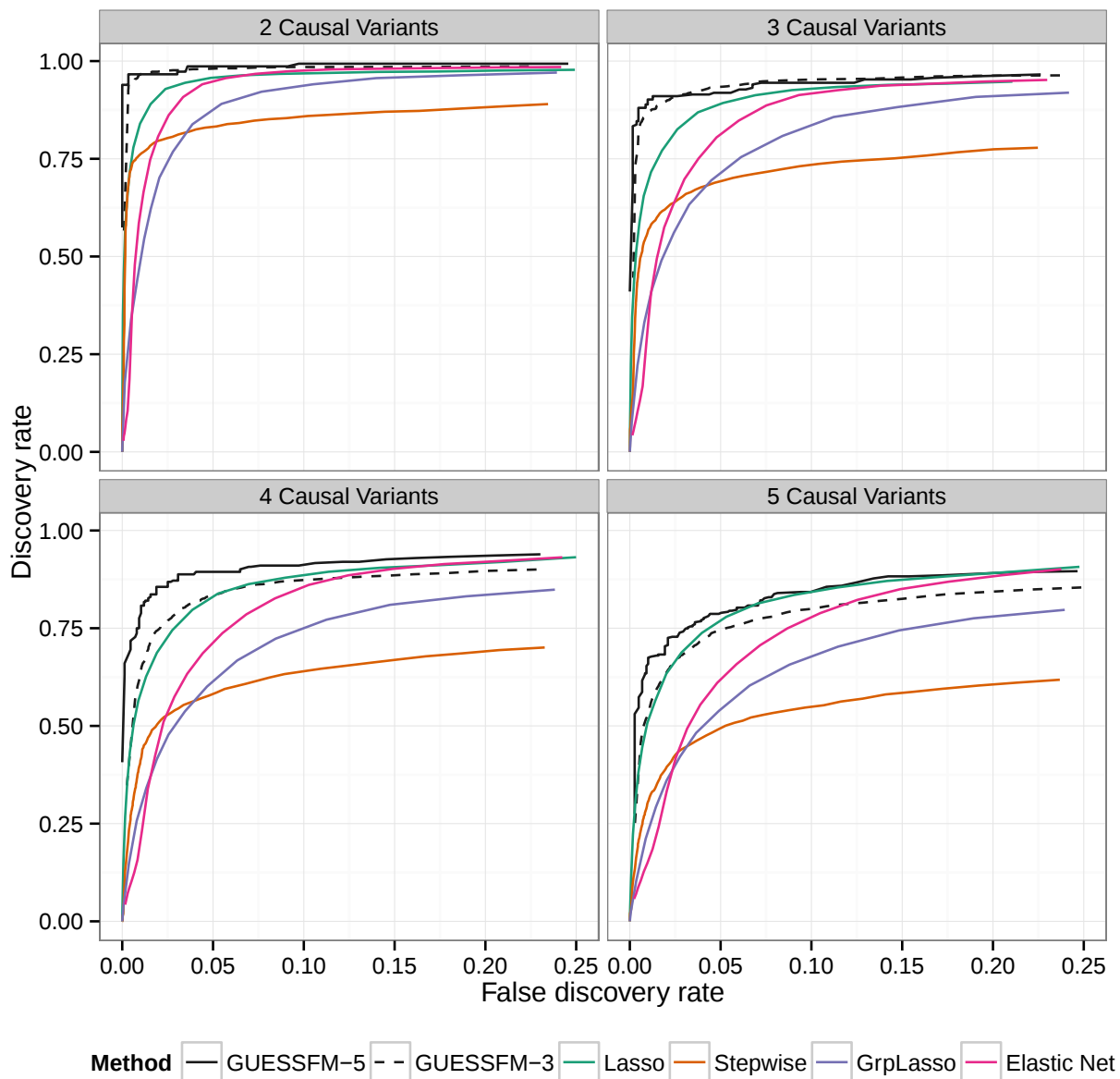
Figure 2. Comparison of several multivariate methods for fine mapping using simulated data. We simulated quantitative phenotype data with between two and five causal variants using genotype data from the T1D dataset for the IL2RA region. The simulated data sets were analysed using forward stepwise regression, GUESSFM, the lasso, the group lasso and the elastic net. GUESSFM produces credible sets for each variant chosen using the snp.picker algorithm described in Materials and Methods. We defined pseudo “credible sets” for the other approaches as the set of SNPs with r^2 > 0.8 with a selected SNP. We calculated the discovery rate (the proportion of causal variants within at least one credible set, y axis) and false discovery rate (proportion of detected variants whose credible sets did not contain any causal variant, x axis) at different thresholds for the stepwise p value, the group marginal posterior probability of inclusion (gMPPI) for GUESSFM and the regularization parameter(s) across simulated datasets (see Methods for details). GUESSFM-3 and GUESSFM-5 refer to GUESSFM run with a prior expectation of three or five causal variants per region, respectively. Results are averaged over 1000 replicates.
