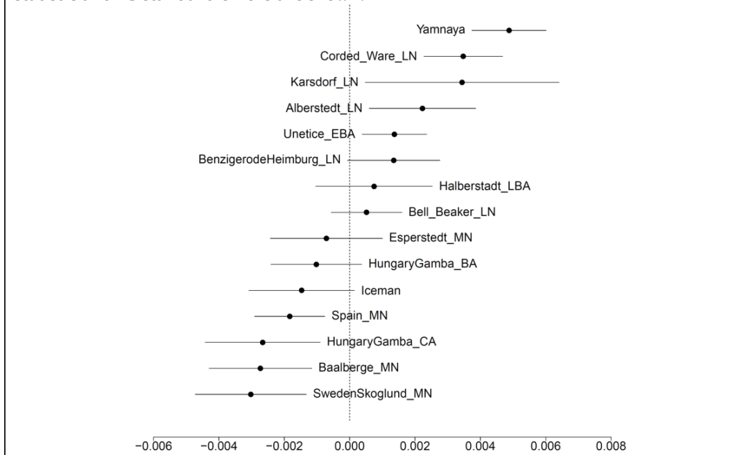
Figure S7.9: The statistic f_4(\text{LBK\_EN, Test; Loschbour, Karelia\_HG}) demonstrates the “eastern” shift of Late Neolithic/Bronze Age Europeans. The estimated value of the statistic and \pm 3 standard errors are shown.
