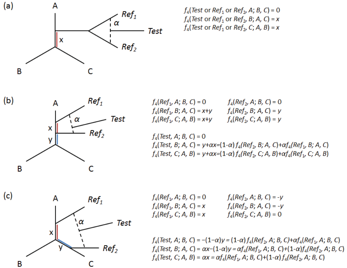
Figure S9.2: Test is a mixture related to two reference populations Ref_1 and Ref_2 . Three possible topologies are shown: (a) Ref_1 and Ref_2 are symmetrically related to A, B, C . (b) Ref_1 and Ref_2 are differentially related to one outgroup A , and symmetrically related to the other two B, C . (c) Ref_1 and Ref_2 are related to two of the outgroups A, C and symmetrically related to the third B . In case (a) all f_4 -statistics involving Test , Ref_1 , Ref_2 are identical and cannot be used to estimate mixture proportions. In cases (b, c) f_4 -statistics involving Test are a weighted average of those involving Ref_1 and Ref_2 .
