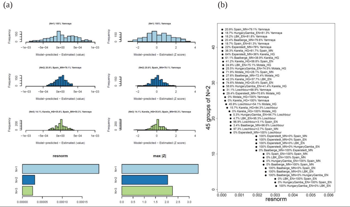
Figure S9.8: Modeling Bell_Beaker_LN as a mixture of earlier populations. (a) We present in the left column a histogram of raw f_4 -statistic residuals and on the right Z-scores for the best-fitting (lowest resnorm ) model at each N . In the bottom row, we show on the left how resnorm and the maximum |Z| score change for different N . (b) resnorm of different N=2 models.
