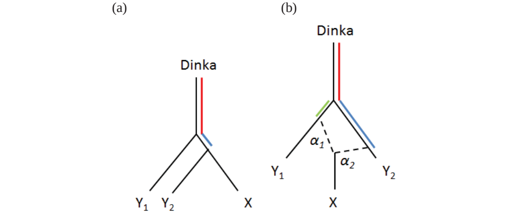
Figure S7.1: “Outgroup” statistic f_3(\text{Dinka}; X, Y) . Panel (a) shows that population Y_2 shares more genetic drift (indicated in blue) with X than Y_1 does. In panel (b), an admixed population X shares genetic drift with Y_1 and Y_2 that is weighted by the admixture proportions \alpha_1 and \alpha_2 .
