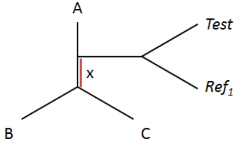
Figure S9.1: If Test and Ref 1 form a clade with respect to the outgroups, then statistics involving either one of them and the outgroups are identical.
