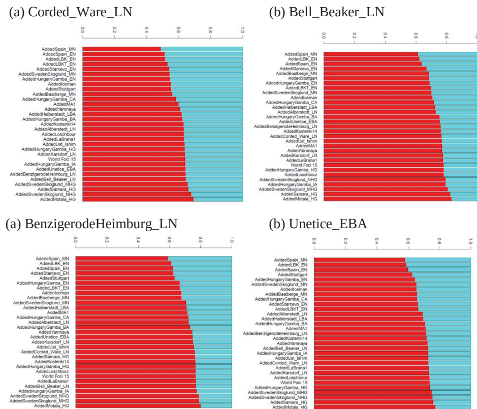
Figure S9.16: Adding EN or MN populations to the set of outgroups reduces the amount of Esperstedt_MN related ancestry (“red”) and increases the amount of Karelia_HG related ancestry (“blue”) inferred for LN/BA populations.
