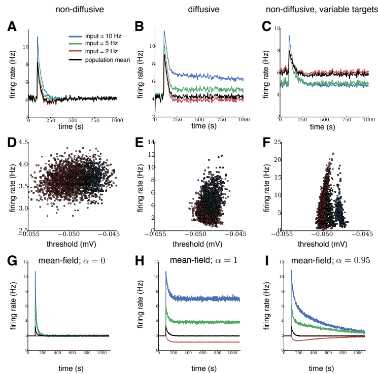
Figure 4. Relative differences between inputs are preserved during diffusive homeostasis. (A-C) Evolution of firing rates in a recurrent network for each input group under diffusive and non-diffusive homeostatic control, and for variable homeostatic targets. Black traces show population activity. Independent Poisson input at the target rate was given to 2000 neurons (red), while two groups of 250 neurons each received elevated Poisson input. The relative rate differences of the groups were only preserved for diffusive homeostasis. (D-F) Final distributions of firing rates versus firing thresholds. (G-I) Evolution of firing rates in a dynamic mean-field population for each input group for purely local ( \alpha = 0 ), purely global ( \alpha = 1 ), and mixed local and global activity read-out ( \alpha = 0.95 ). Black traces show population activity. Input at the target rate is given to 2000 neurons (red), while two groups of 250 neurons each receive elevated input.
