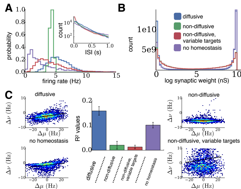
Figure 7. Diffusive homeostasis retains its properties in networks with STDP. (A) Distributions of steady-state firing rates after homeostasis and STDP. (Inset) Distribution of inter-spike intervals at the steady-state (log scale). (B) Distributions of steady-state synaptic weights after homeostasis and STDP. (C) Mean response linearity (measured by R^2 values) for networks with STDP and each case of homeostasis ( n=9 networks, error bars represent one standard deviation). Surrounding plots show firing rate changes \Delta\nu of all neurons following input changes \Delta\mu for an example network in each case (black line shows linear fit).
