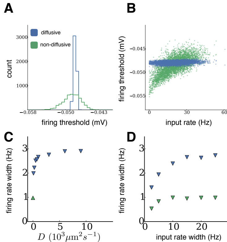
Figure 3. Steady-state firing thresholds of diffusive and non-diffusive homeostasis. (A) Distributions of firing thresholds after homeostasis from network simulations, receiving independent Poisson input drawn from a Gaussian distribution. (B) Steady-state firing thresholds plotted against external inputs received during homeostasis. (C) Width of the steady-state firing rate distribution as the diffusion coefficient D is varied ( D = 1000 \mu\text{m}^2 \text{s}^{-1} in panels A-B). (D) Width of the steady-state firing rate distribution as the input rate width is varied, for networks with diffusive ( D = 1000 \mu\text{m}^2 \text{s}^{-1} ) and non-diffusive homeostasis (input rate width = 10 Hz in panels A-B).
