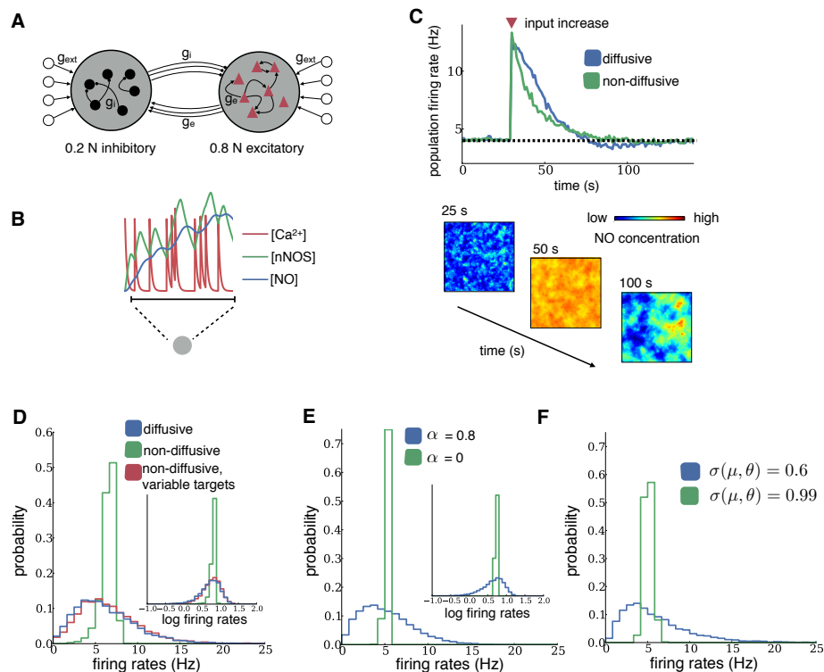
Figure 1. Steady-state behavior of diffusive and non-diffusive homeostasis.
