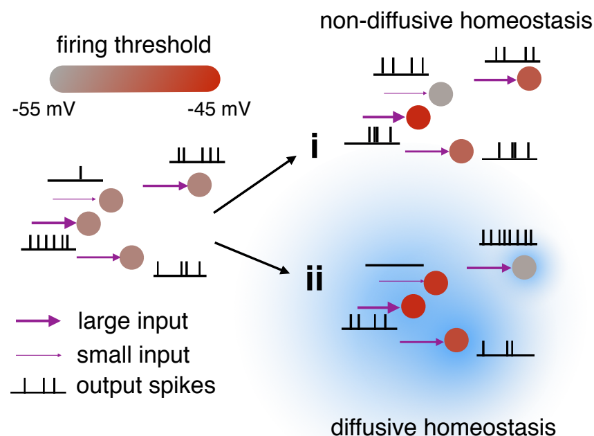
Figure 2. Illustration of the effects of non-diffusive (i) and diffusive (ii) homeostasis. Non-diffusive homeostasis adjusts each neuron's threshold (red color bar) according to its input to give identical firing rates, while diffusive homeostasis induces correlations (blue cloud) in the thresholds of neighboring neurons, thereby maintaining diverse firing rates.
