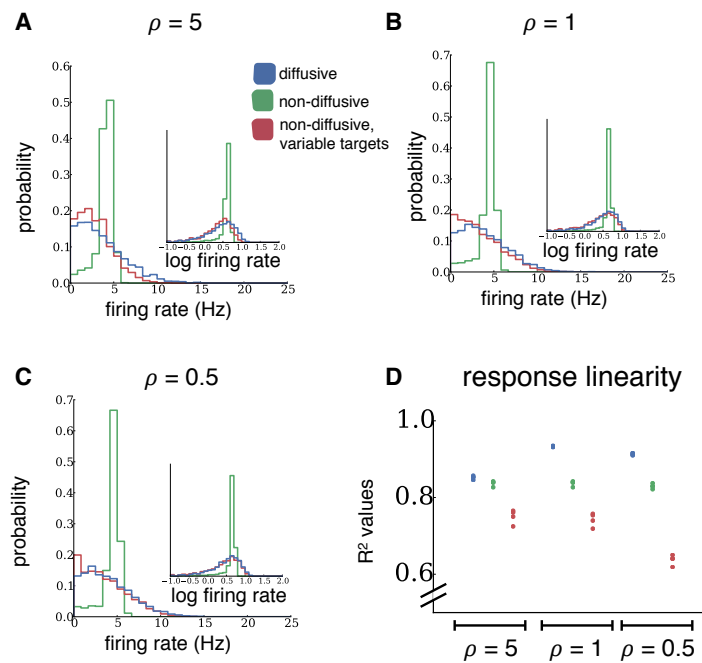
Figure S1. Linearity of network responses in networks with spatially restricted connection probabilities. These results qualitatively agree with those for the random networks used throughout the study. The simulations shown here were identical to those in Figs. 1D and 5 of the main text, but the connection probability between neurons had a Gaussian shape. \rho , the ratio of the connectivity range and the diffusive range, is varied across a wide range of values ( \rho=0.5, 1.0, 5.0 ). (D) Each point represents the R^2 value of a linear fit as in Figs. 5A-C, for one network.
