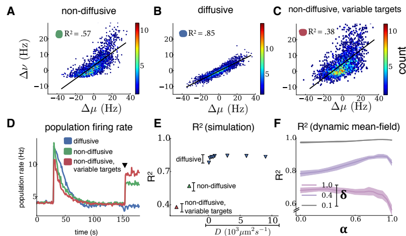
Figure 5. Diffusive homeostasis enables linear network responses. (A-C) Firing rate changes \Delta\nu of all neurons following input changes \Delta\mu . Black lines show linear fits, with corresponding R^2 values inset. (D) Population activity before and after input change (black triangle). (E) Linearity of the population response to a change of inputs as the diffusion coefficient D is varied ( D = 1000 \mu\text{m}^2 \text{s}^{-1} in panel B). (F) Linearity of the population response to a change of inputs in the mean-field analysis as \alpha is varied, shown for different input distribution widths \delta . Shaded regions correspond to one standard deviation, averaged over 25 independent network trials for each value of \delta .
