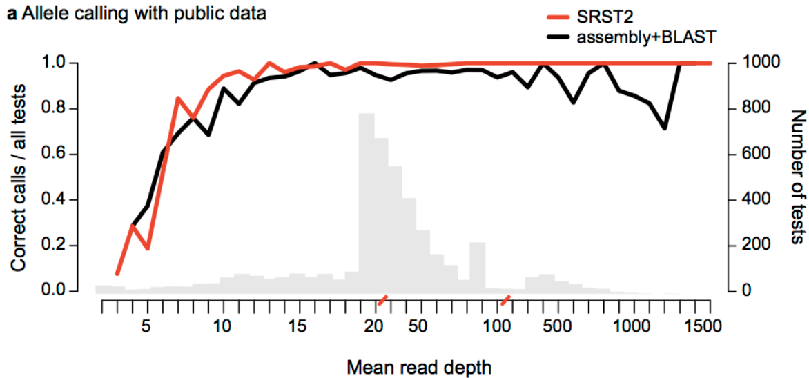
Figure 3. Overall accuracy of SRST2 allele calling and gene detection
